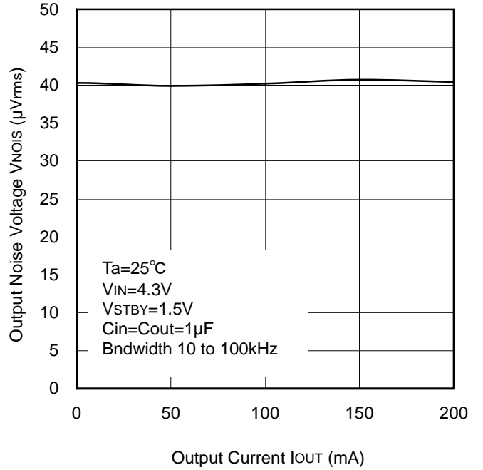
Figure 83. Output Noise Voltage vs. Output Current
