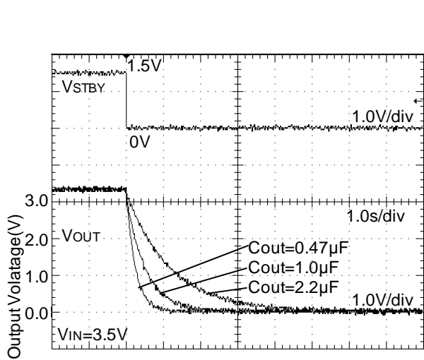
Figure 91. Discharge Time (ROUT=none)
