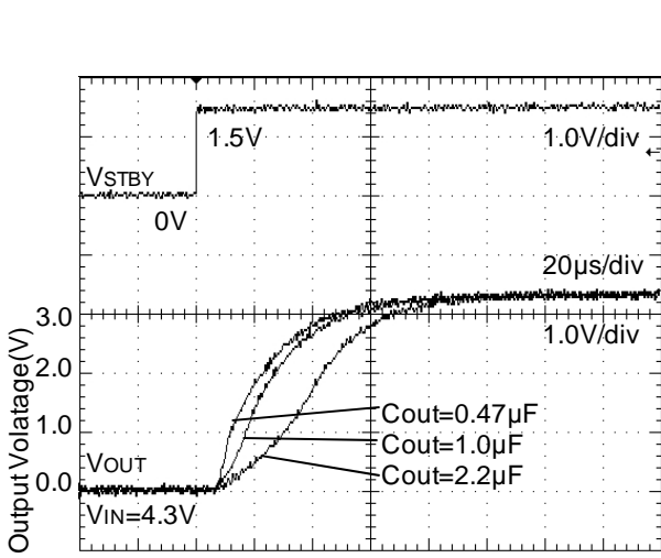
Figure 89. Startup Time (ROUT=none)
