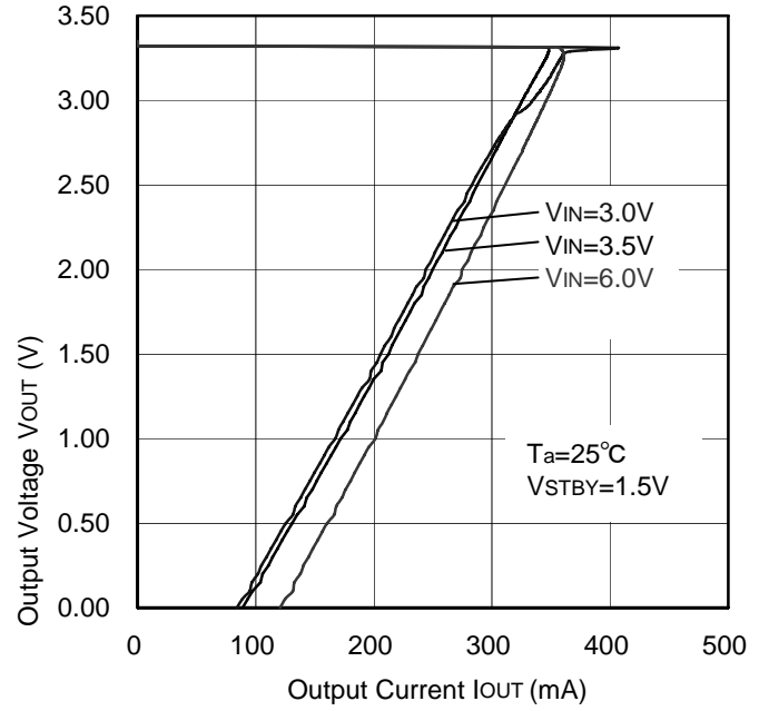
Figure 75. OCP Threshold
