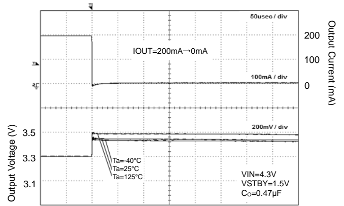
Figure 20. Load Response
