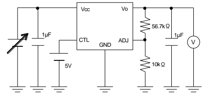
Measurement Circuit of Figure 6
