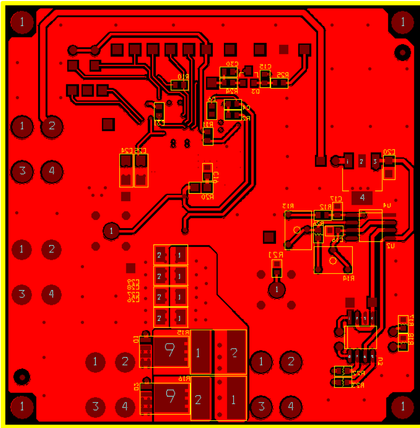
Figure 31. Evaluation Board Bottom Layer Copper
