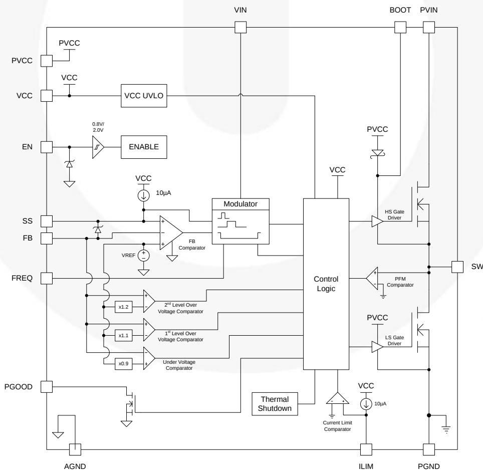
Figure 2. Block Diagram
