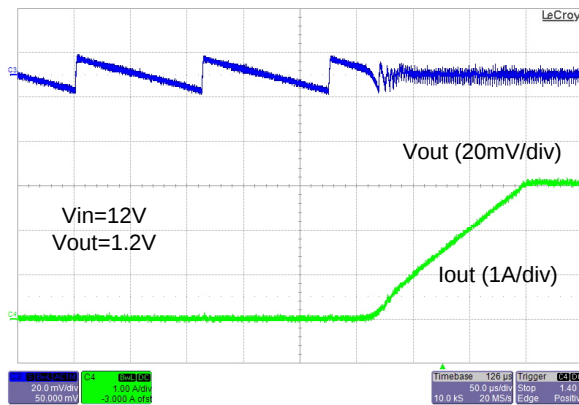
Figure 17. FAN2306M Transition from DCM to CCM
