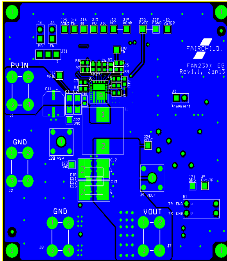
Figure 28. Evaluation Board Top Layer Copper
