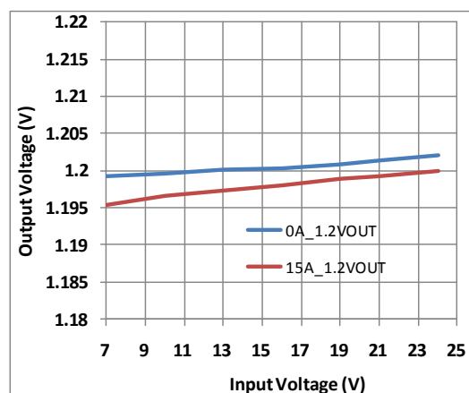
Figure 15. Line Regulation
