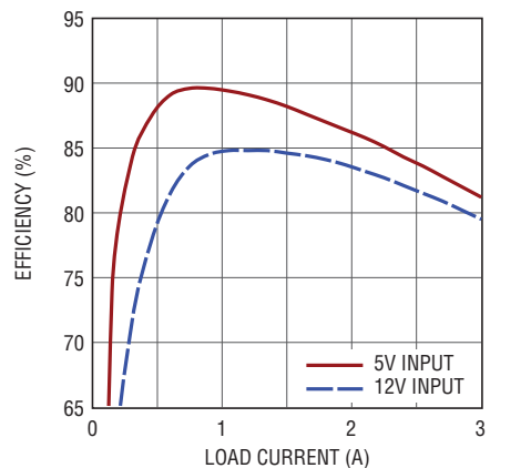
Output Efficiency vs Load Current
