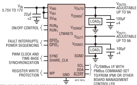
Dual 9A \mu Module Regulator with Digital Interface for Control and Monitoring*
