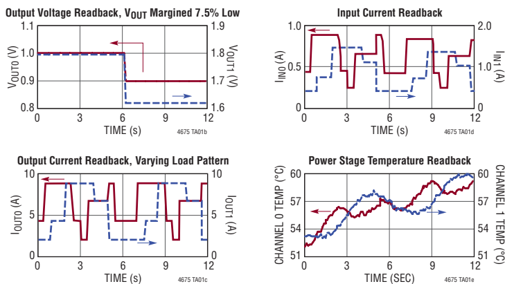
Using PMBus and LTpowerPlay to Monitor Telemetry and Margin V OUT0 /V OUT1 During Load Pattern Tests. 10Hz Polling Rate. 12V IN
