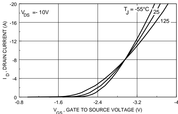
Figure 5. Transfer Characteristics.
