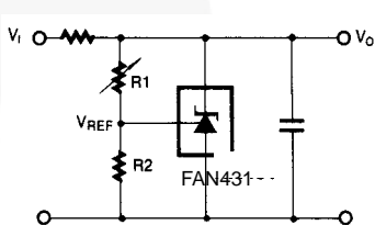
Figure 5. Shunt Regulator
