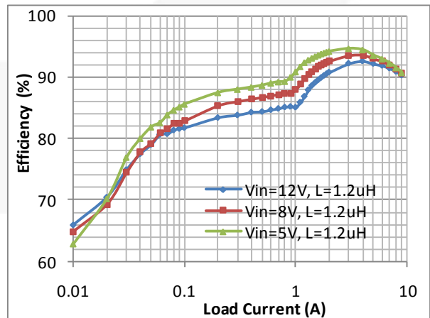
Figure 10. FAN2306MA Efficiency vs. Load Current with V_{OUT}=1.2\text{ V} and f_{SW}=500\text{ kHz}
