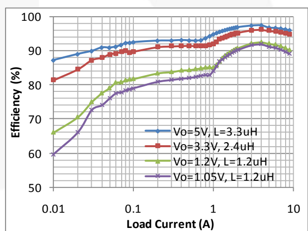
Figure 8. FAN2306MA Efficiency vs. Load Current with V_{IN}=12\text{ V} and f_{SW}=500\text{ kHz}
