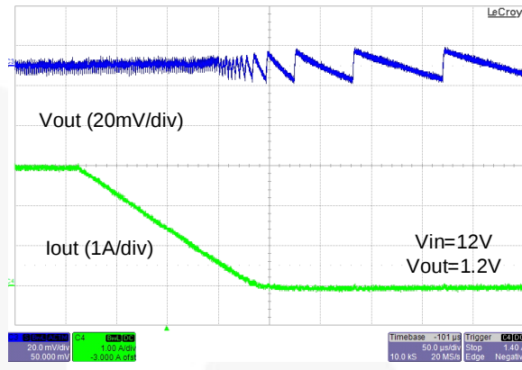
Figure 18. FAN2306MA Transition from CCM to DCM
