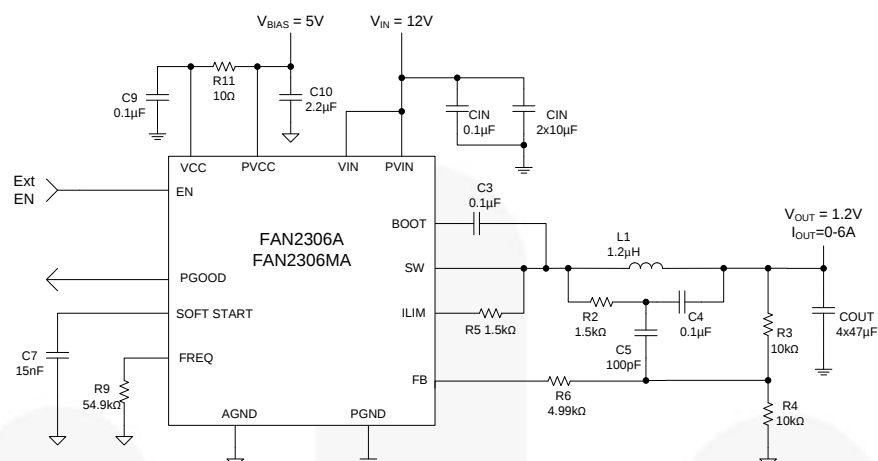
Figure 1. Typical Application
