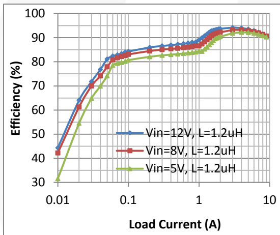
Figure 7. FAN2306A Efficiency vs. Load Current with V_{OUT}=1.2\text{ V} and f_{SW}=500\text{ kHz}
