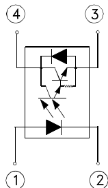
① Anode ② Cathode ③ Emitter ④ Collector
