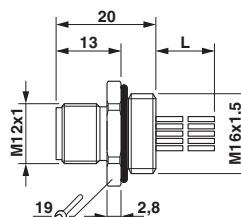
Dimensional drawing
