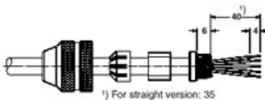
Strip conductor, widen shield and lay around the shielding ring, cut off projecting mesh.
