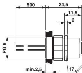
M12 flush-type plug, can be positioned
