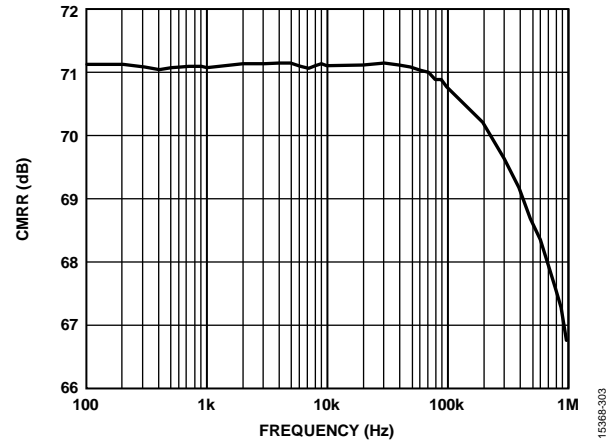
Figure 37. CMRR vs. Frequency, V_{IO} = 3.3\text{ V} , V_{REF} = 5\text{ V} , 25^\circ\text{C}
