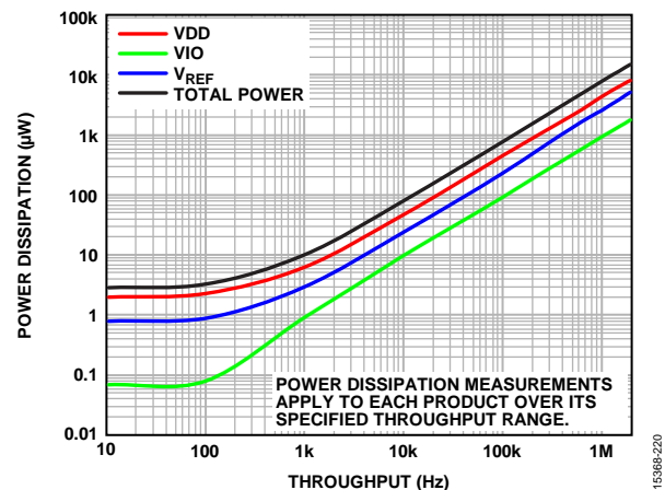
Figure 46. Power Dissipation vs. Throughput, V_{IO} = 1.8\text{ V} , V_{REF} = 5\text{ V}
