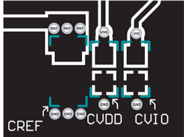
Figure 66. Example Layout of the AD4001 (Bottom Layer)
