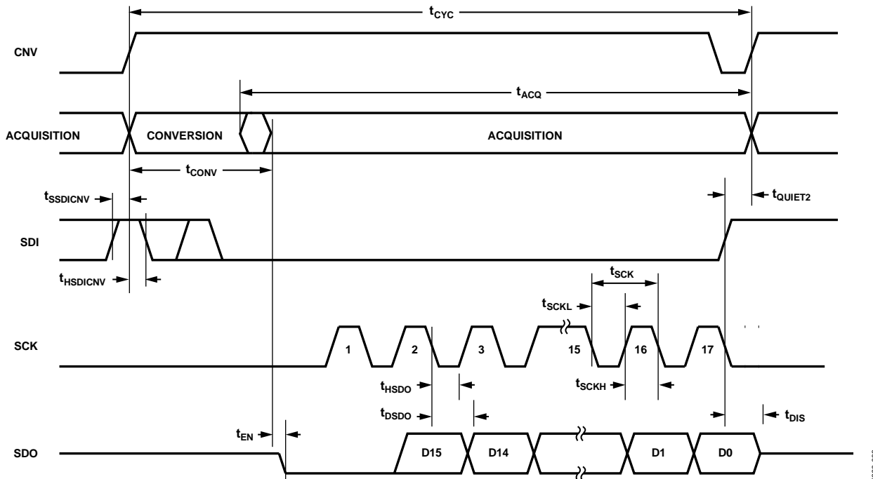
Figure 62. CS Mode, 4-Wire with Busy Indicator Serial Interface Timing Diagram
