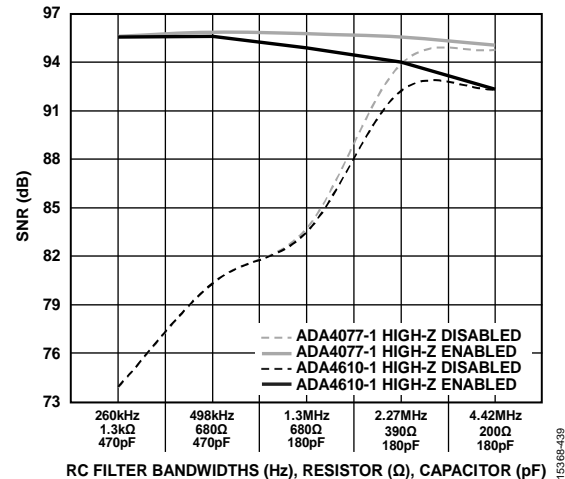
Figure 43. SNR vs. RC Filter Bandwidths for Various Precision ADC Drivers, V_{REF} = 5\text{ V} , f_{IN} = 1\text{ kHz} (Turbo Mode On, High-Z Enabled/Disabled), V_{IO} = 3.3\text{ V}
