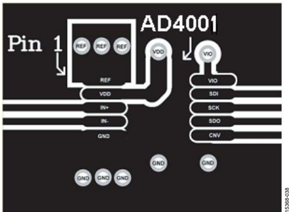
Figure 65. Example Layout of the AD4001 (Top Layer)
