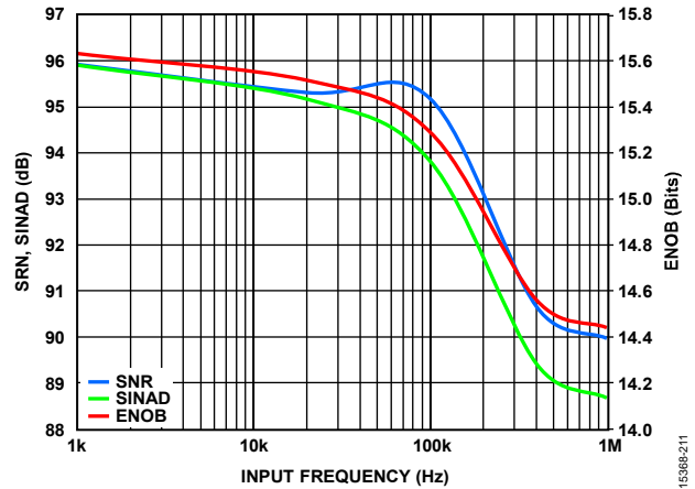
Figure 38. SNR, SINAD, and ENOB vs. Input Frequency
