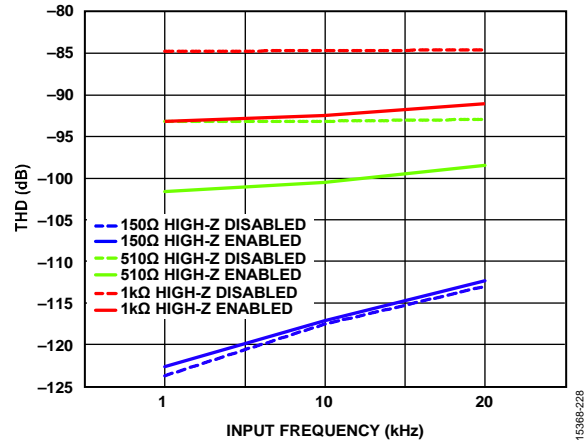
Figure 42. THD vs. Input Frequency for Various Source Impedance, V_{REF} = 5\text{ V}
