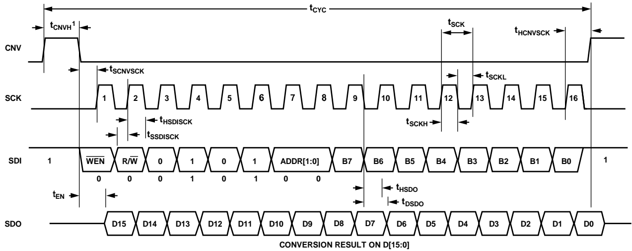
Figure 48. Register Write Timing Diagram
