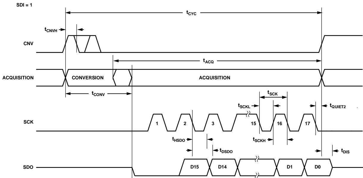
Figure 56. \overline{CS} Mode, 3-Wire with Busy Indicator Serial Interface Timing Diagram (SDI High)
