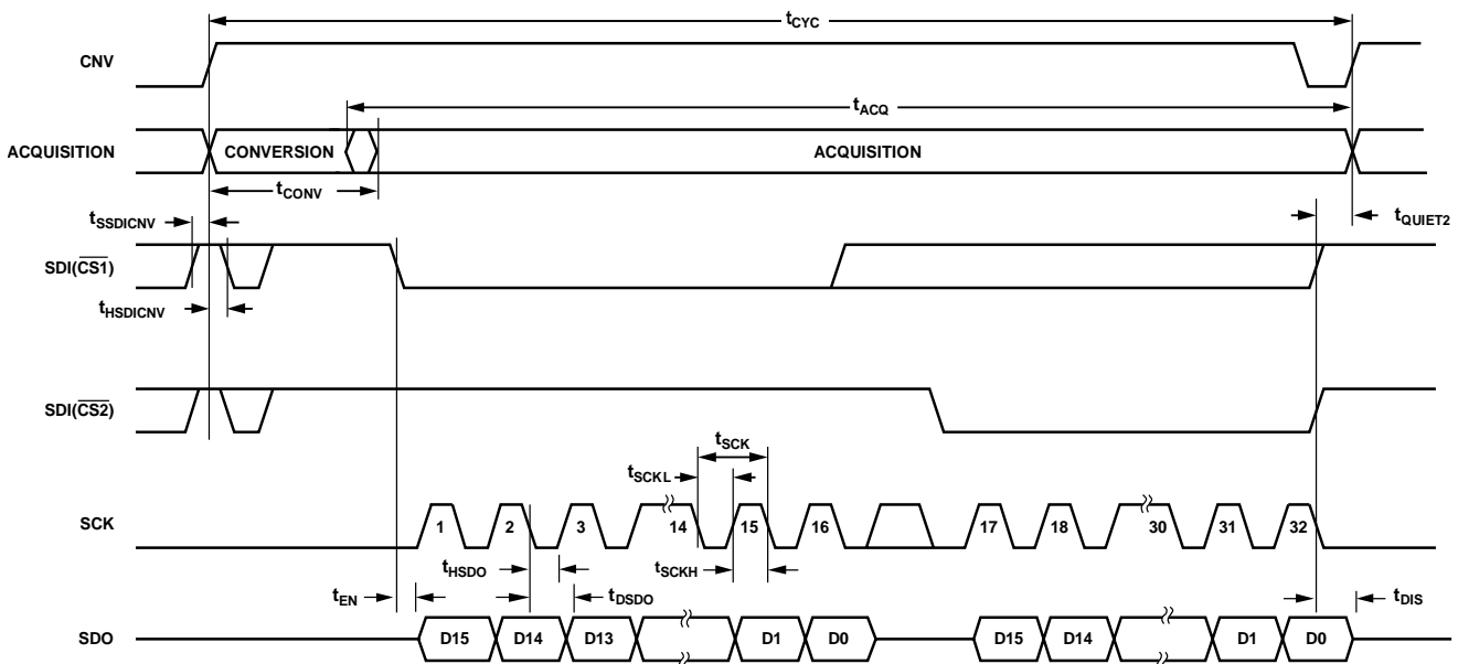
Figure 60. CS Mode, 4-Wire Without Busy Indicator Serial Interface Timing Diagram
