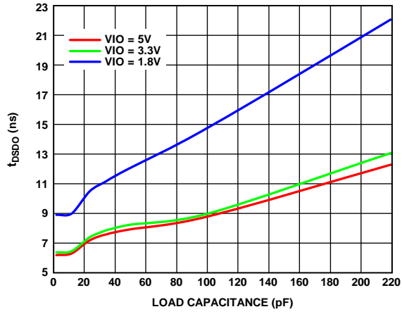
Figure 29. t_{DSDO} vs. Load Capacitance
