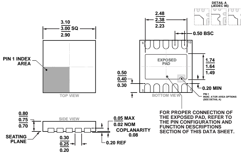
Figure 68. 10-Lead Lead Frame Chip Scale Package [LFCS] 3 mm x 3 mm Body and 0.75 mm Package Height (CP-10-9) Dimensions shown in millimeters
