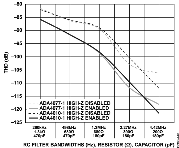
Figure 44. THD vs. RC Filter Bandwidths for Various Precision ADC Drivers, V_{REF} = 5\text{ V} , f_{IN} = 1\text{ kHz} (Turbo Mode On, High-Z Enabled/Disabled)
