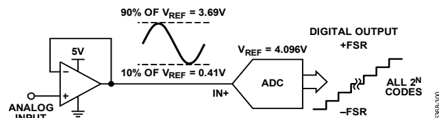
Figure 40. Span Compression
