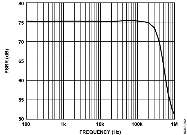
Figure 45. PSRR vs. Frequency, V_{IO} = 3.3\text{ V} , V_{REF} = 5\text{ V}
