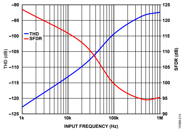
Figure 39. THD and SFDR vs. Input Frequency
