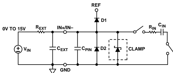
Figure 36. Equivalent Analog Input Circuit
