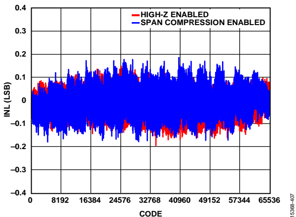
Figure 7. INL vs. Code, High-Z and Span Compression Enabled, VREF = 5 V
