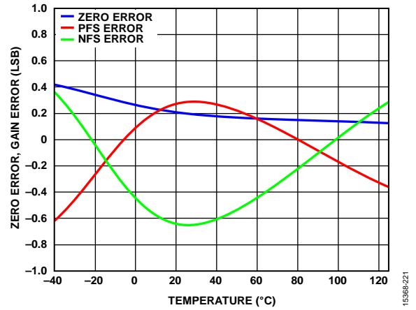
Figure 26. Zero Error and Gain Error vs. Temperature, Positive Full Scale (PFS) and Negative Full Scale (NFS)
