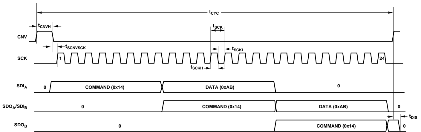
Figure 49. Register Write Timing Diagram, Daisy-Chain Mode
