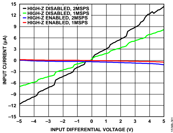
Figure 41. Input Current vs. Input Differential Voltage, V_{IO} = 3.3\text{ V} , V_{REF} = 5\text{ V}
