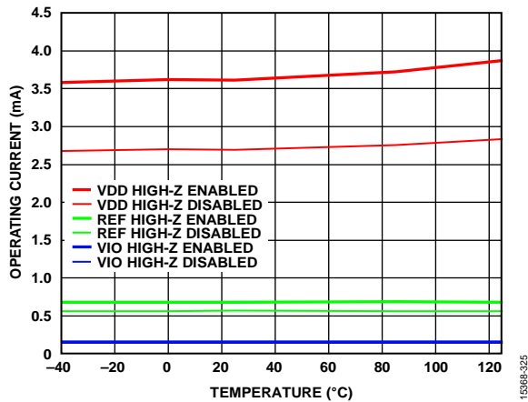
Figure 25. Operating Current vs. Temperature, AD4005, 1 MSPS
