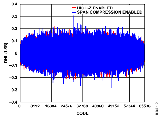
Figure 10. DNL vs. Code, High-Z and Span Compression Enabled, VREF = 5 V
