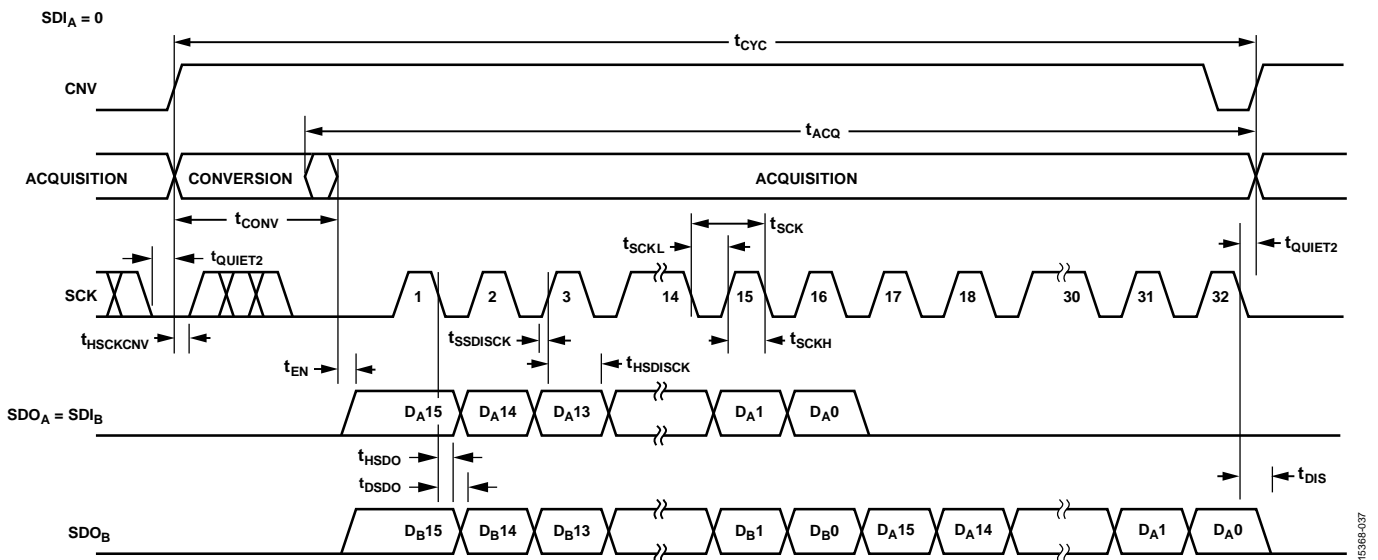
Figure 64. Daisy-Chain Mode Serial Interface Timing Diagram
