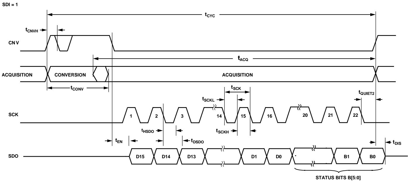
Figure 50. \overline{CS} Mode, 3-Wire Without Busy Indicator Serial Interface Timing Diagram, Including Status Bits (SDI High)
