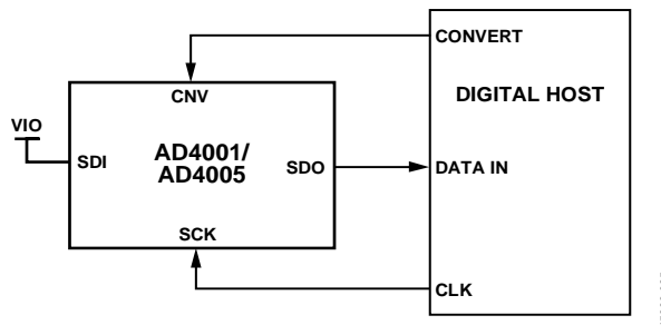
Figure 53. \overline{CS} Mode, 3-Wire Without Busy Indicator Connection Diagram (SDI High)
