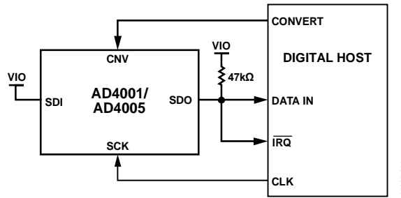
Figure 55. \overline{CS} Mode, 3-Wire with Busy Indicator Connection Diagram (SDI High)
