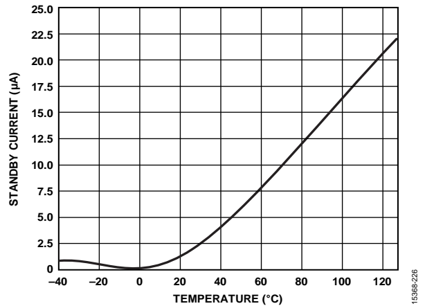
Figure 28. Standby Current vs. Temperature
