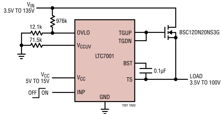
High Side Switch with VCCUV and OVLO
