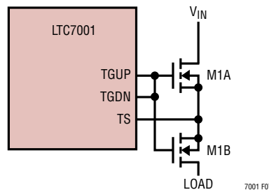
Figure 7. Protecting Load from Voltage Drops on V_{IN}
