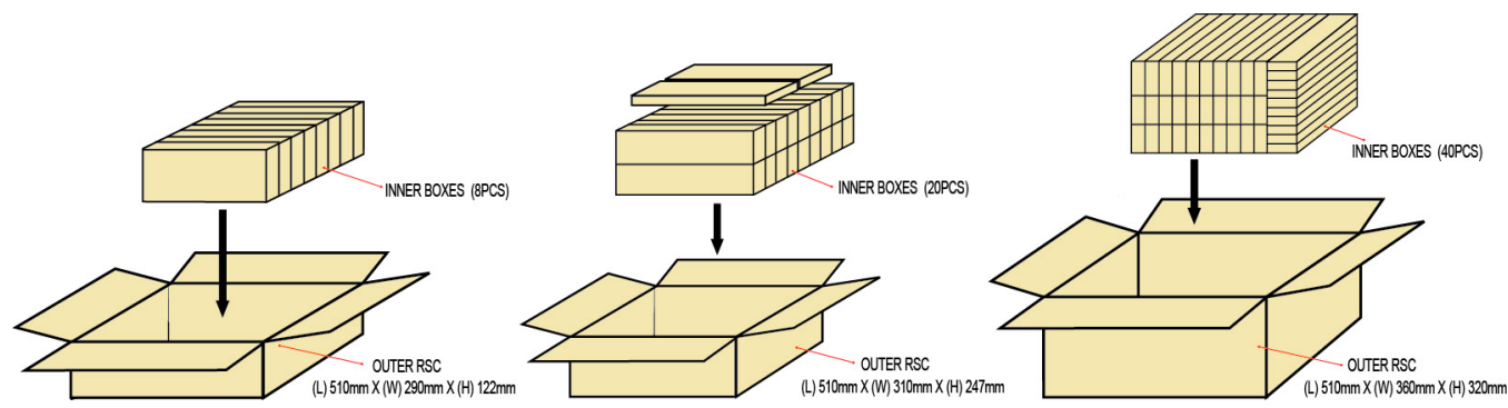
Figure 13. Dimensions for outer box packaging for LUXEON CoB with CrispColor Technology.
