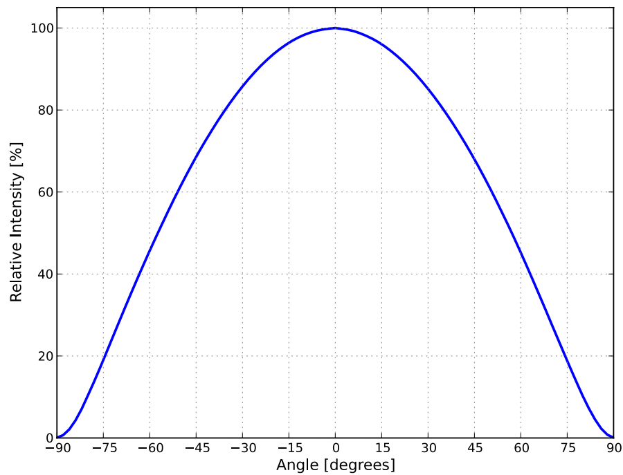
Figure 5. Typical radiation pattern for LUXEON CoB with CrispColor Technology at specified test current, T_j=85^{\circ}\text{C} .
