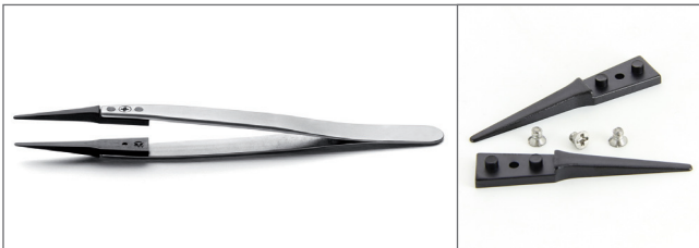
242CFR.SA - 242CPR.SA - 242SVR.SA Tips: straight, narrow, flat, round. OAL: 130mm A242CF - A242CP - A242SV Replacement tip set. OAL: 40mm. ESD safe
