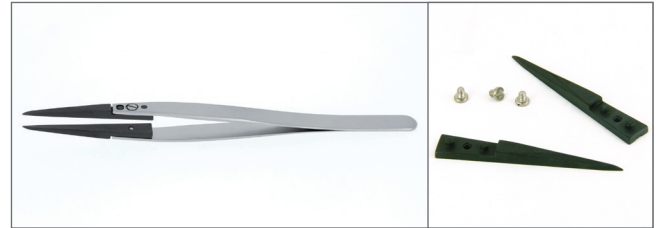
72ZJ.SA Tips: straight, strong, pointed, superior finish. OAL: 135mm A72ZJ Replacement tip set. OAL: 45mm. ESD safe
