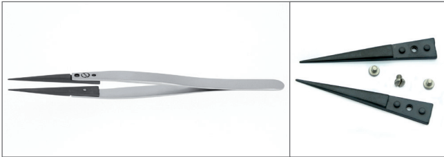
71ZJ.SA Tips: straight, thin, fine, superior finish. OAL: 135mm A71ZJ Replacement tip set. OAL: 45mm. ESD safe
