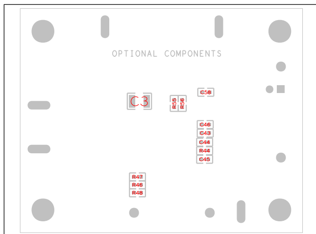
MAXM17502 EV Kit—Bottom
