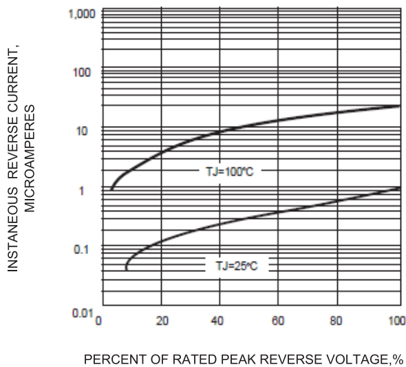
FIG.3-TYIACL REVERSE CHARACTERISTICS
