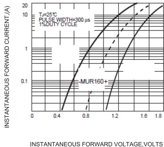
FIG.4-TYPICAL FORWARD CHARACTERISTICS
