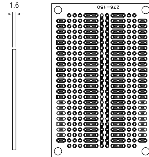
Copper Surface
