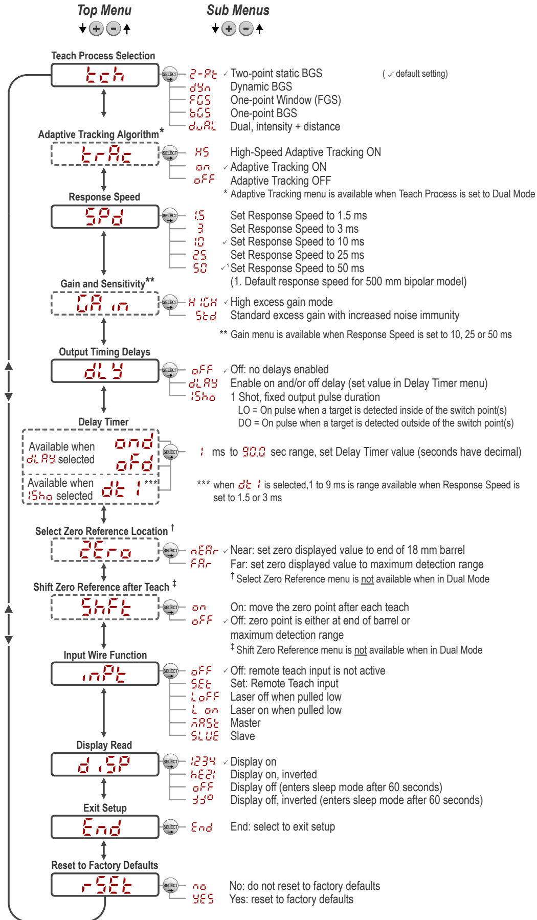
Figure 10. Sensor Menu Map—Channel 1
