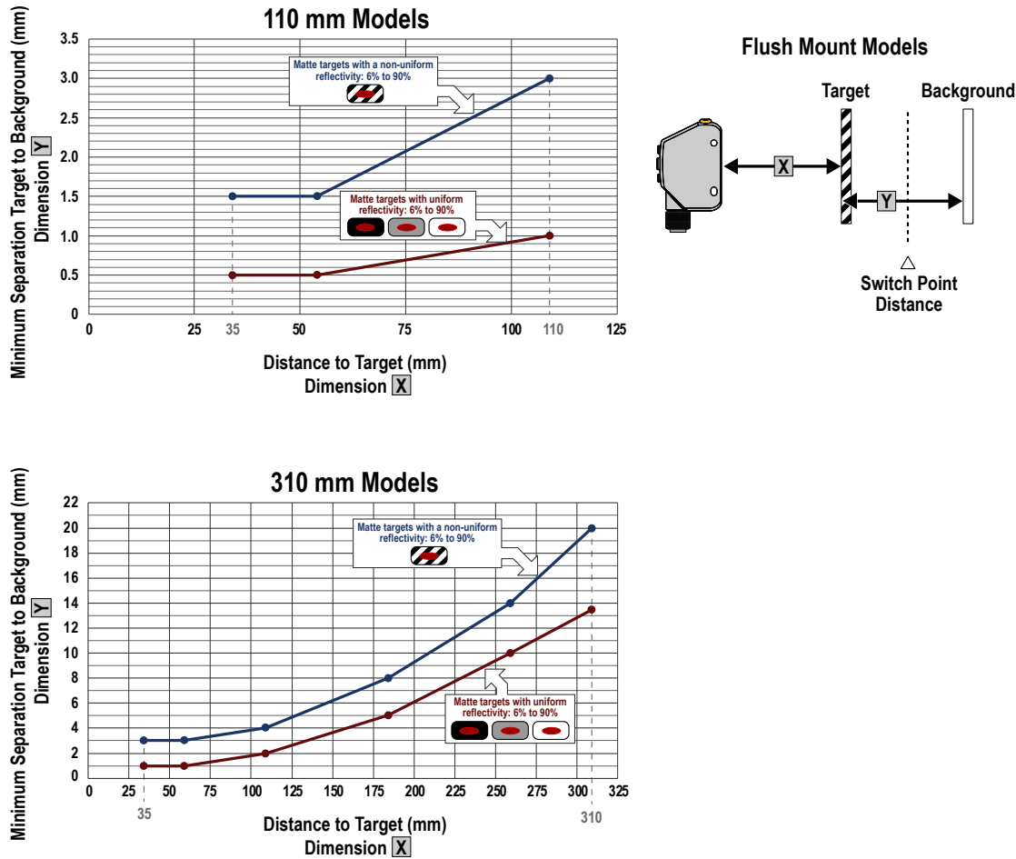
Figure 12. Minimum Object Separation Distance (90% to 6% reflectance)
