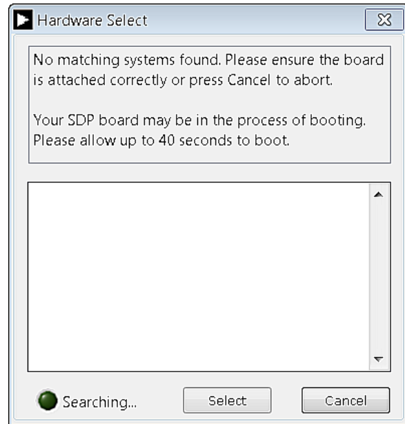
Figure 2. Connectivity Error
