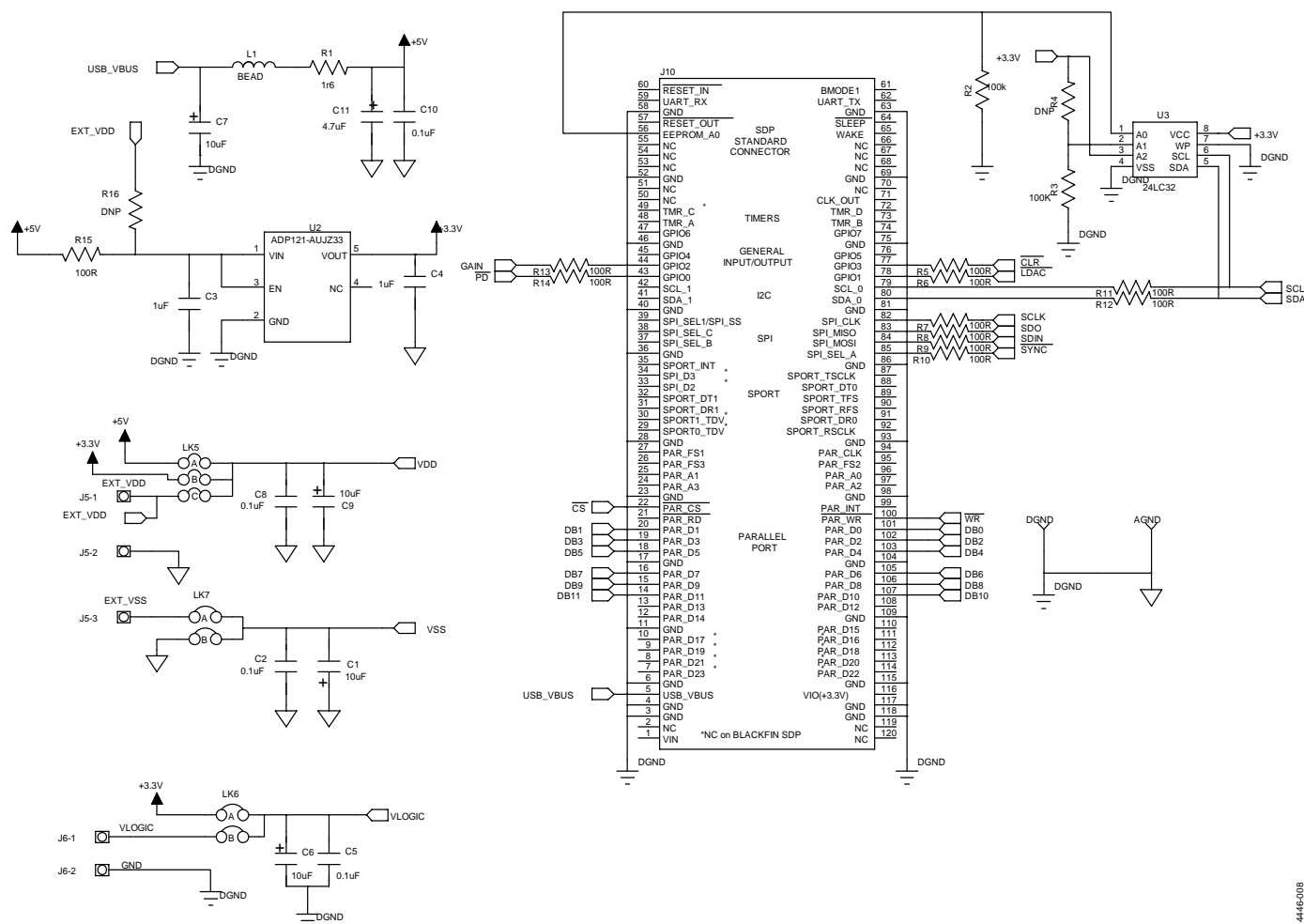
Figure 8. EVAL-MBnanoDAC-SDZ Motherboard SDP-B Connector and Power Supply
