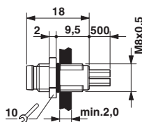
Dimensional drawing
