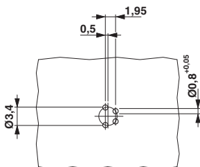
Drilling diagram
