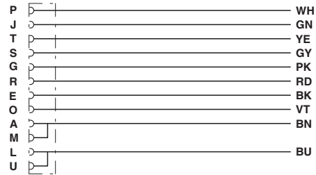
Contact assignment of the M16 socket
