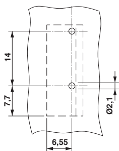
Drilling diagram
