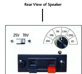
Rear View of Speaker
