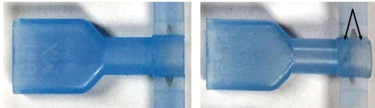
Current 16-14 AWG standard flare part (shown here with optional carrier strip attached)
