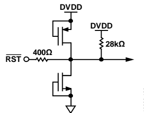
Figure 26. \overline{RST} Equivalent Circuit
