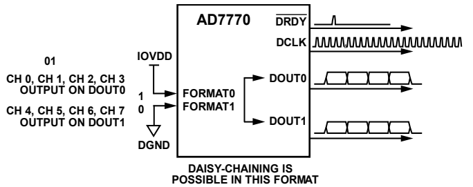
Figure 113. FORMATx Pin Configuration—FORMAT0 = 1, FORMAT1 = 0
