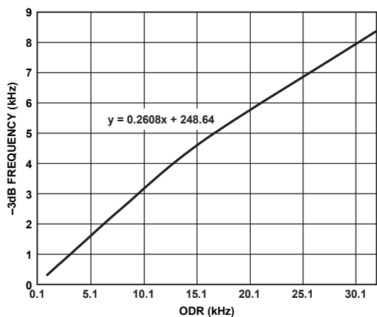
Figure 111. -3 dB Correction Factor
