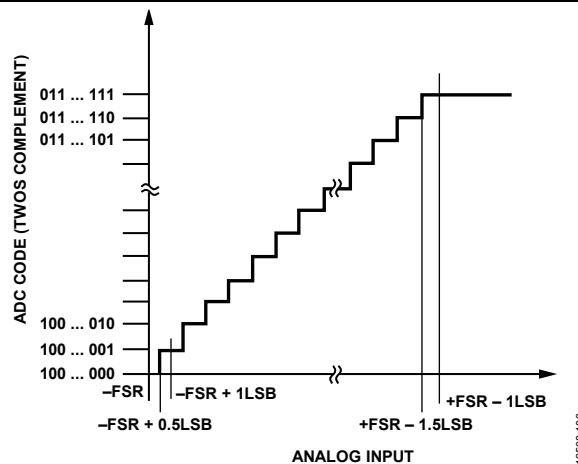
Figure 91. Transfer Function
