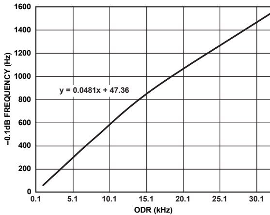
Figure 110. -0.1 dB Correction Factor
