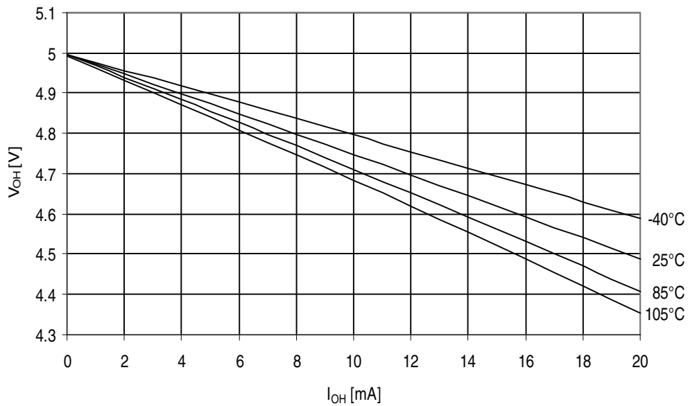
Figure 32-197. ATmega329PA - 105°C: I/O Pin Output Voltage vs. Source Current, Port B ( V_{CC} = 5V )
