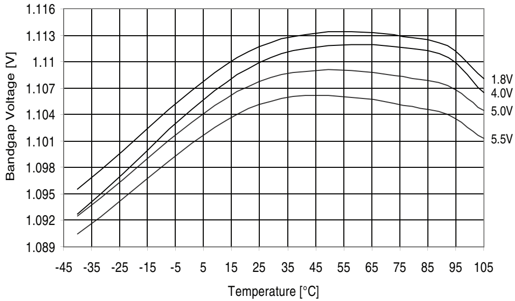
Figure 32-395. ATmega3290PA: Bandgap Voltage vs. Temperature
