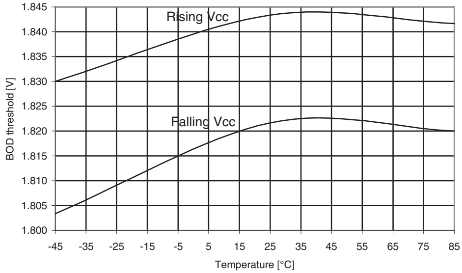
Figure 31-468. Atmel ATmega649P: BOD Thresholds vs. temperature (BOD level is 1.8V).
