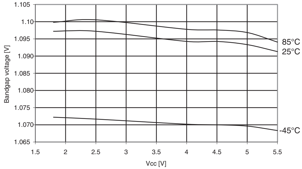
Figure 31-43. Atmel ATmega169A: Bandgap voltage vs. V_{CC} .
