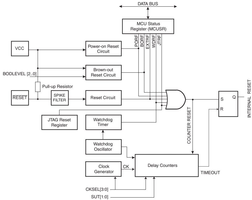
Figure 11-1. Reset logic.
