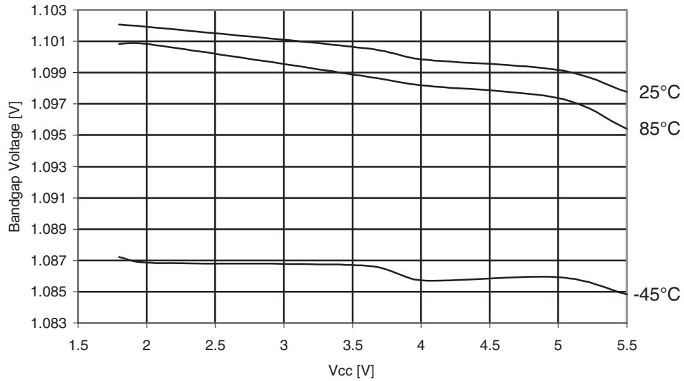
Figure 31-469. ATmega649P: Bandgap voltage vs. V_{CC} .
