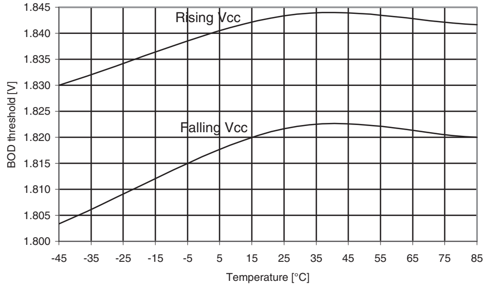
Figure 31-590. Atmel ATmega6490P: BOD Thresholds vs. temperature (BOD level is 1.8V).
