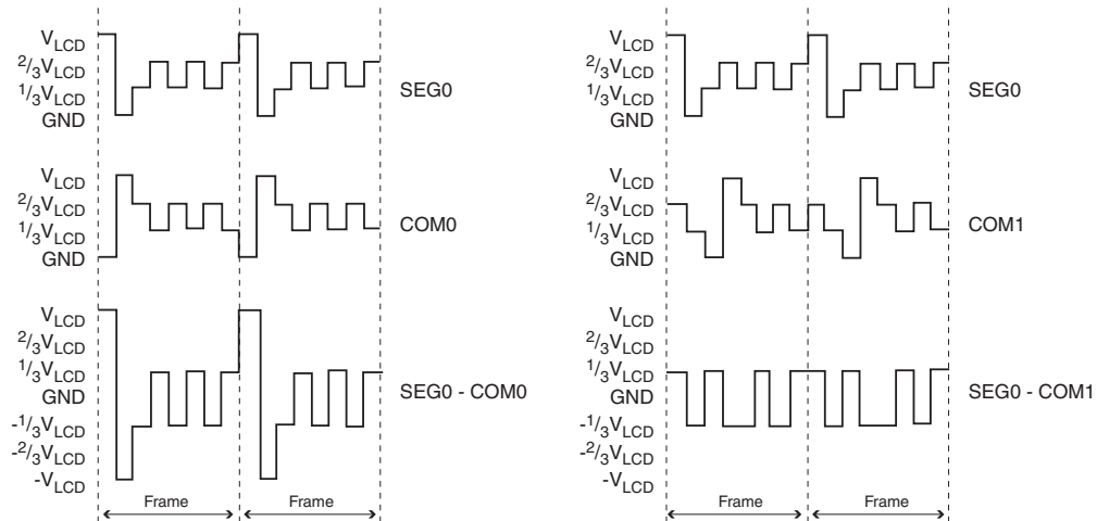
Figure 24-6. Driving a LCD with four common terminals.
