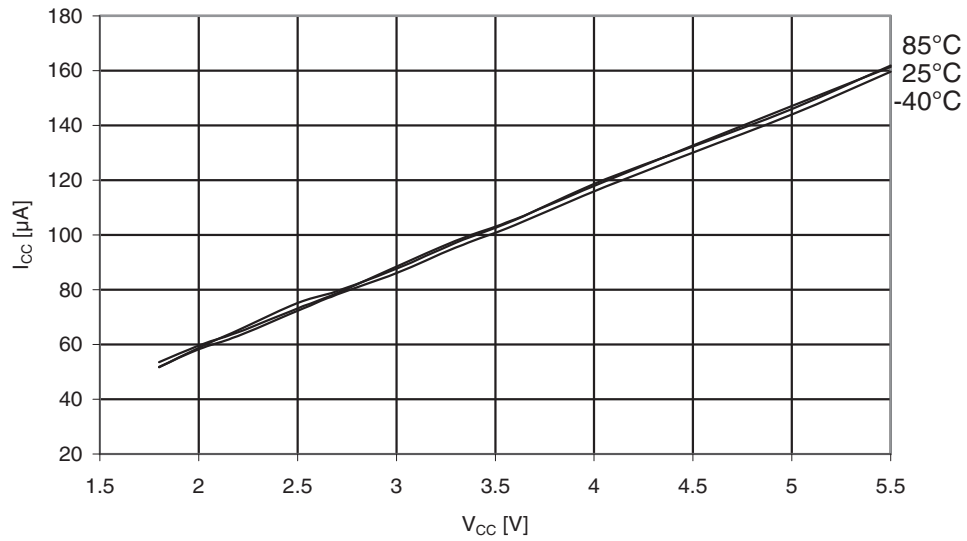
Figure 31-178. ATmega329A: AREF external reference current vs. V_{CC} .
