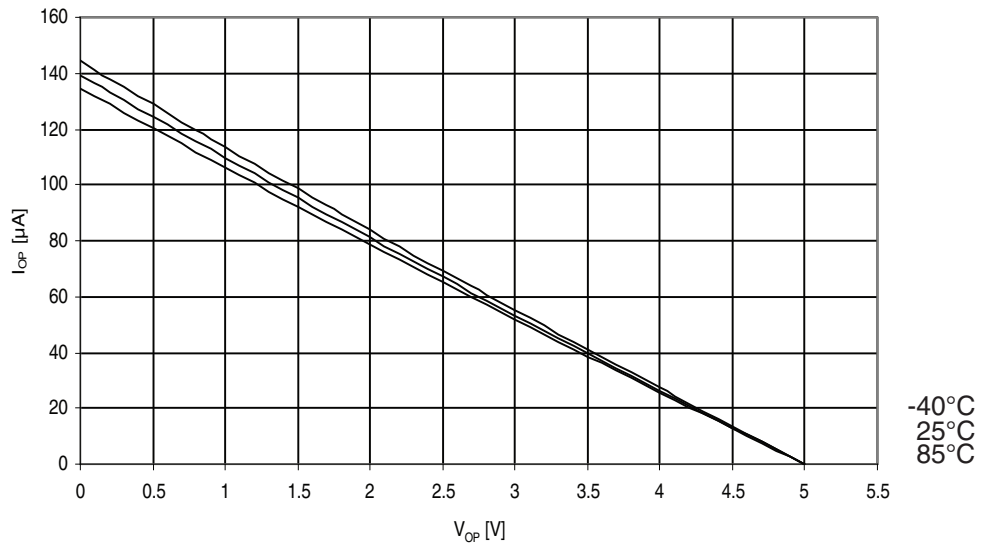
Figure 31-320. Atmel ATmega3290PA: I/O pin pull-up resistor current vs. input voltage ( V_{CC} = 5V ).
