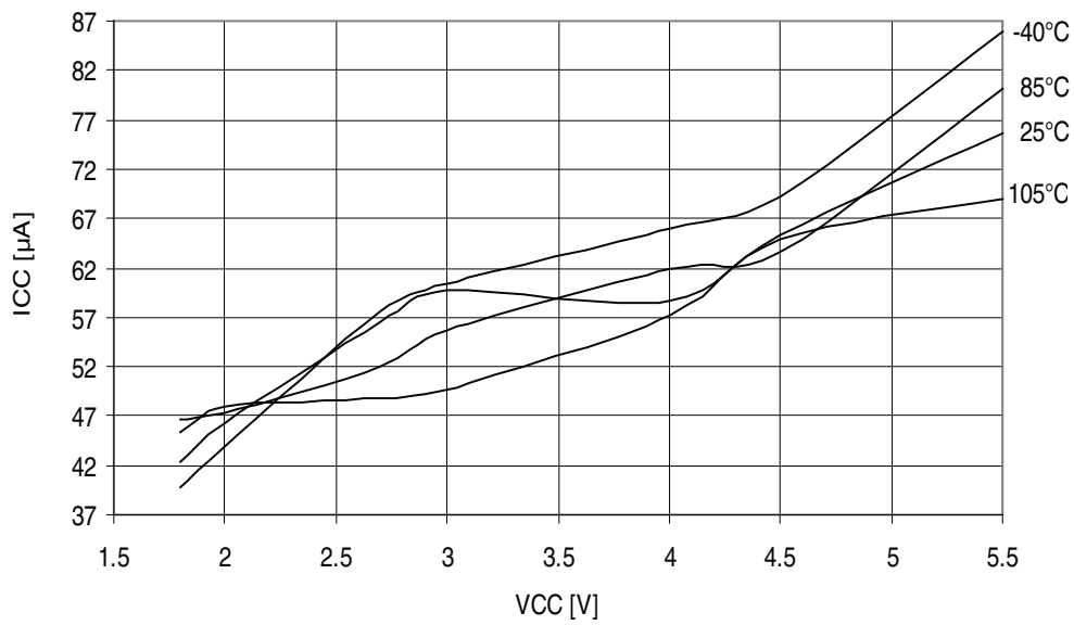
Figure 32-294. ATmega3290A - 105°C: Analog Comparator Current vs. V_{CC}
