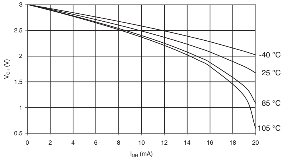
Figure 32-323. ATmega3290PA-105°C: I/O Pin Output Voltage vs. Source Current, Port B ( V_{CC} = 3V )
