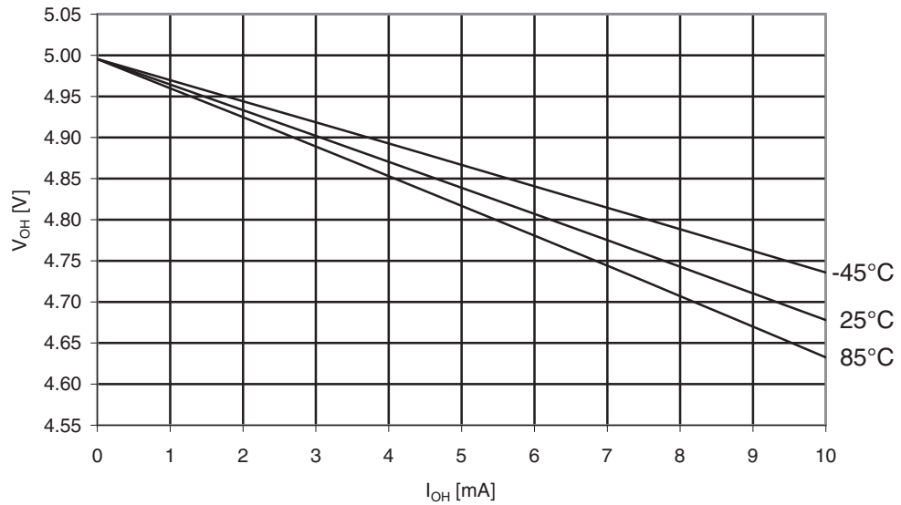
Figure 31-84. ATmega169PA: I/O pin output voltage vs. Source current, ports A, C, D, E, F, G ( V_{CC} = 5V ).
