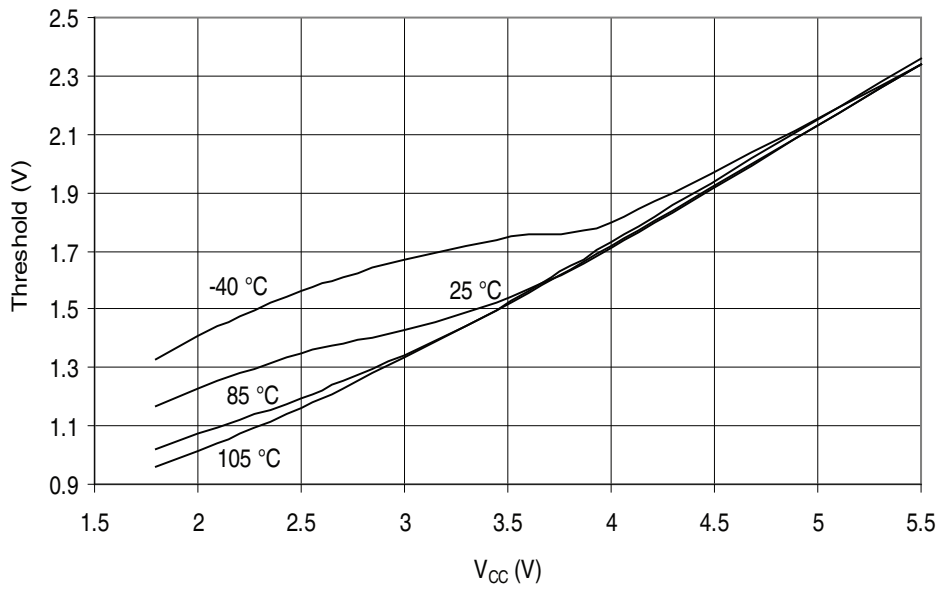
Figure 32-272. ATmega3290A - 105°C: Reset Input Threshold Voltage vs. V_{CC} ( V_{IH,Reset} , Reset Pin Read as "1")
