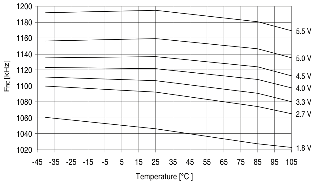
Figure 32-280. ATmega3290A - 105°C: Watchdog Oscillator Frequency vs. Temperature
