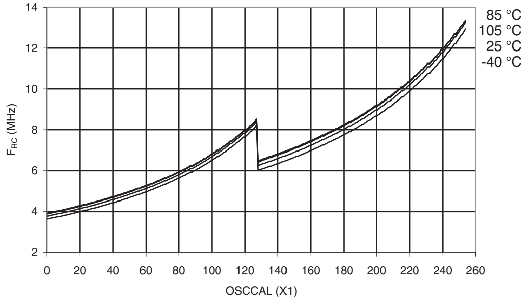
Figure 32-342. ATmega3290PA-105°C: Calibrated RC Oscillator Frequency vs. Oscscal Value
