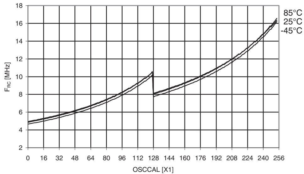
Figure 31-475. ATmega649P: Calibrated 8MHz RC oscillator frequency vs. Oscscal value.
