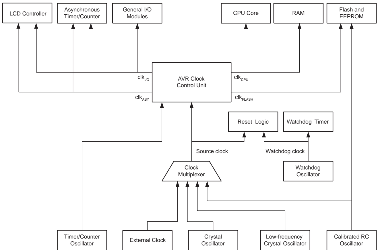
Figure 9-1. Clock distribution.
