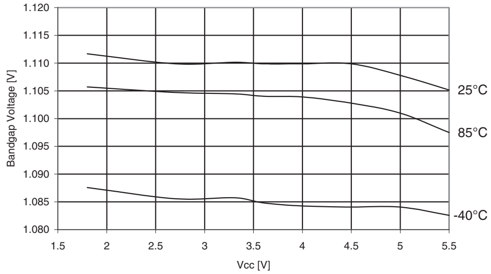
Figure 31-347. ATmega3290PA: Bandgap voltage vs. V_{CC} .
