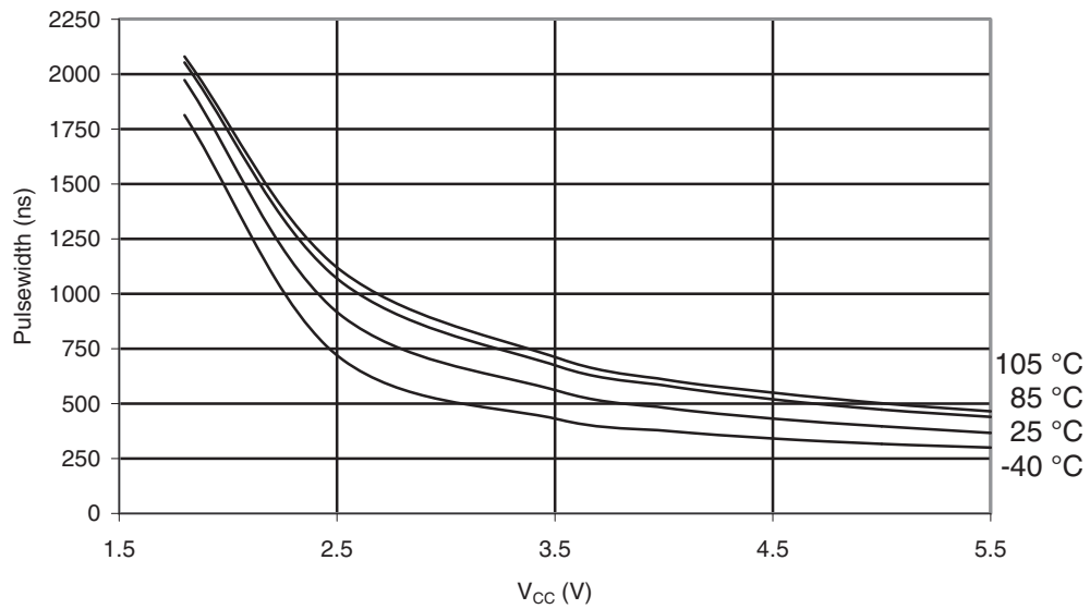
Figure 32-351. ATmega3290PA-105°C: Minimum Reset Pulse Width vs. V_{CC}
