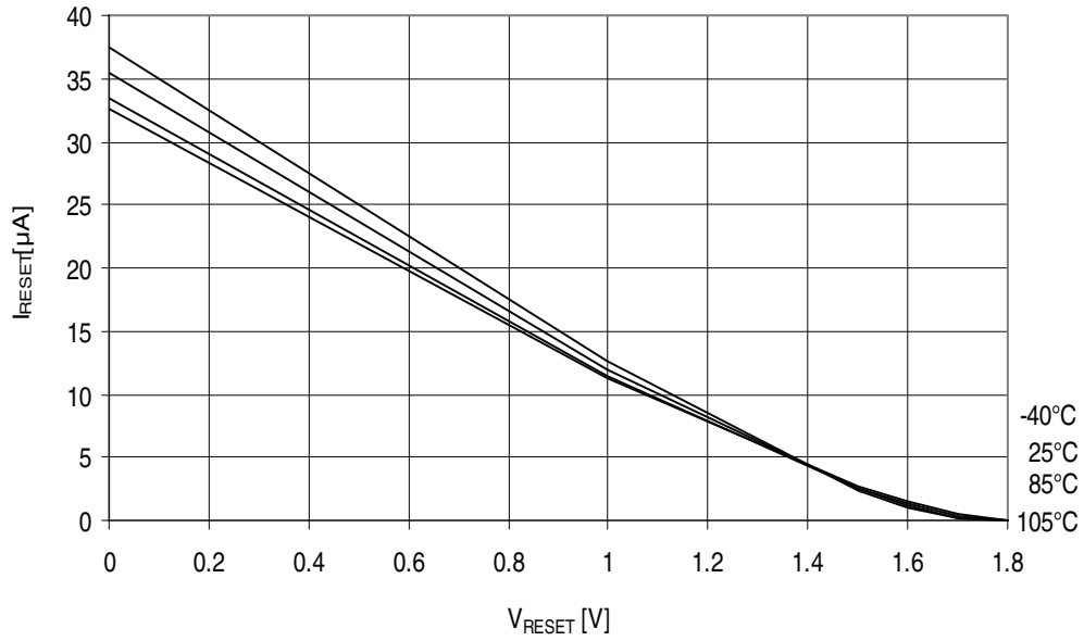
Figure 32-372. ATmega3290PA - 105°C: Reset Pull-up Resistor Current vs. Reset Pin Voltage ( V_{CC} = 1.8V )
