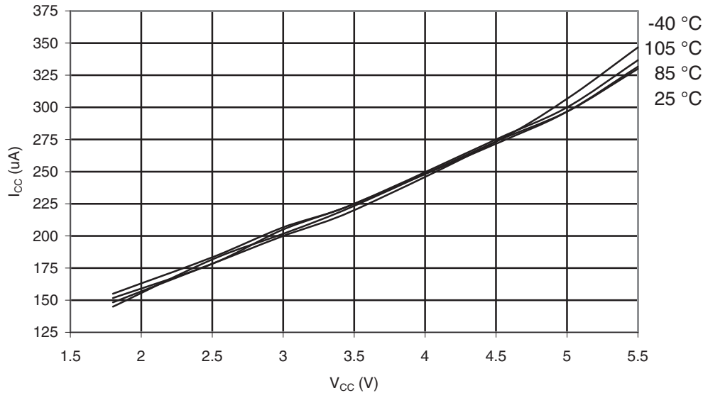
Figure 32-344. ATmega3290PA-105°C: Active supply current with ADC vs. V_{CC}
