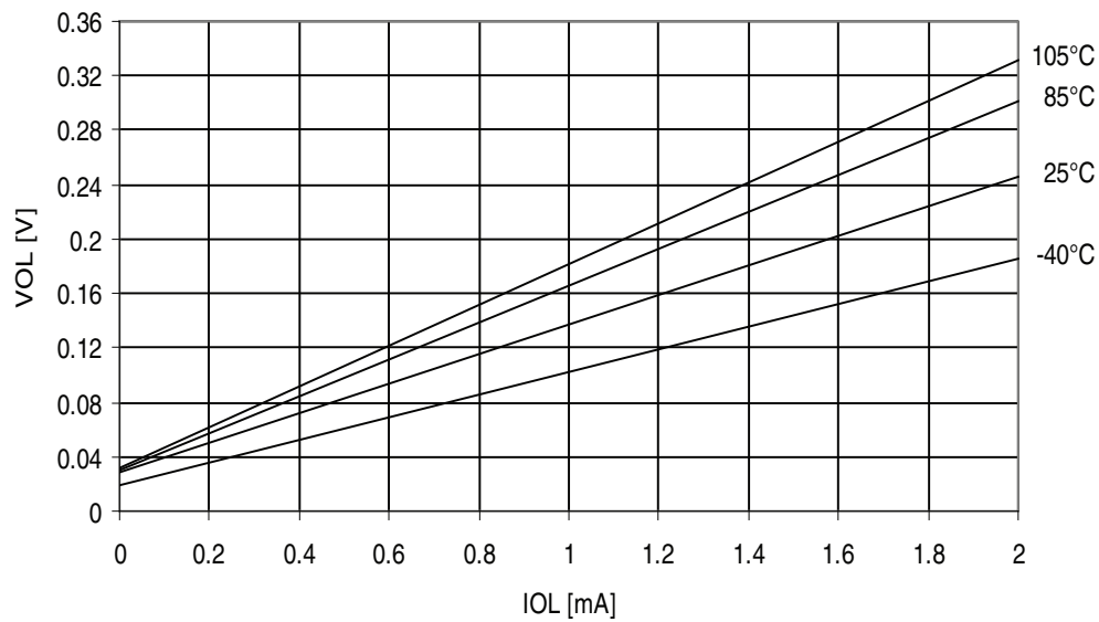
Figure 32-381. ATmega3290PA - 105°C ATmega3290PA - 105°C: I/O Pin Output Voltage vs. Sink Current, Ports A, C, D, E, F, G ( V_{CC} = 1.8V )
