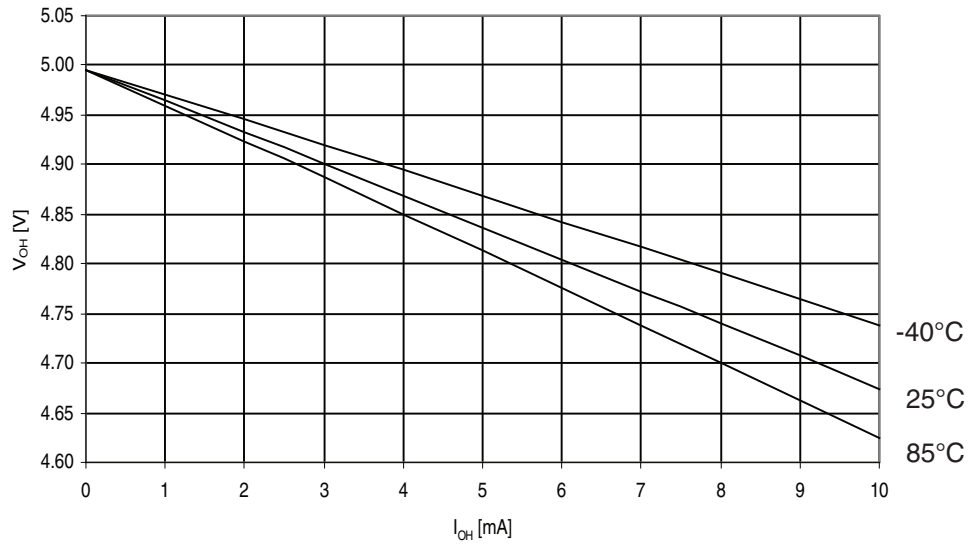
Figure 31-146. ATmega329A: I/O pin output voltage vs. source current, ports A, C, D, E, F, G ( V_{CC} = 5V ).
