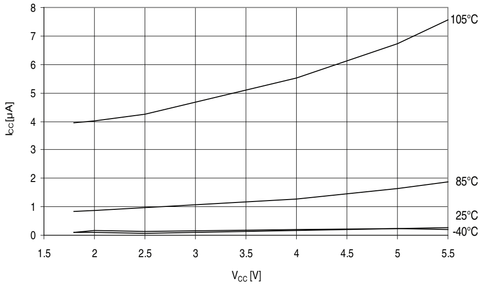
Figure 32-184. ATmega329PA - 105°C: Power-down Supply Current vs. V_{CC} (Watchdog Timer Disabled)
