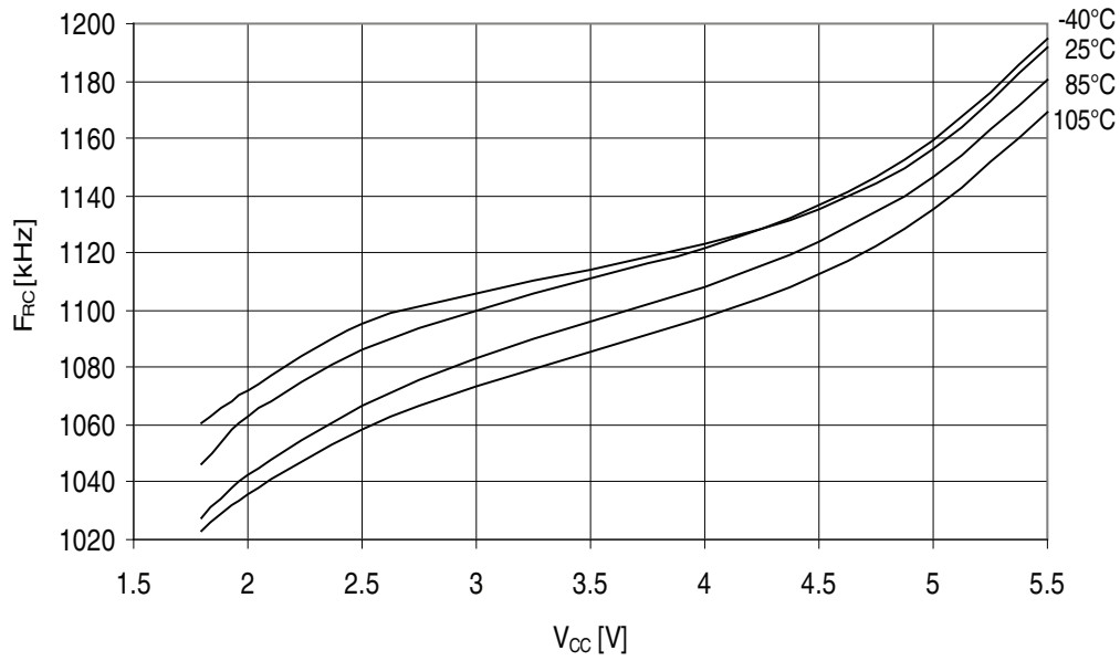
Figure 32-218. ATmega329PA - 105°C: Watchdog Oscillator Frequency vs. V CC
