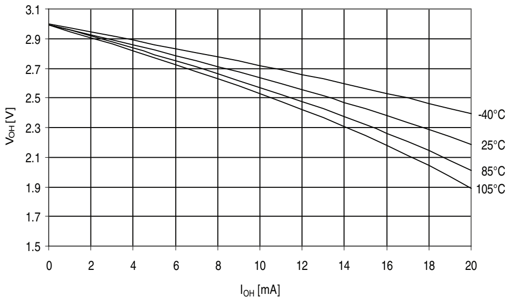
Figure 32-377. ATmega3290PA - 105°C: I/O Pin Output Voltage vs. Source Current, Port B ( V_{CC} = 3V )
