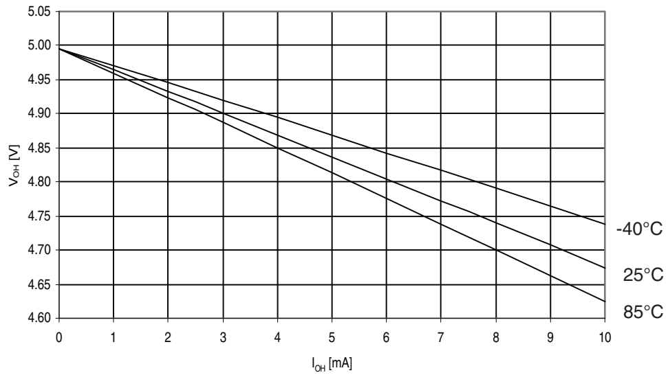
Figure 31-266. ATmega3290A: I/O pin output voltage vs. source current, ports A, C, D, E, F, G ( V_{CC} = 5V ).
