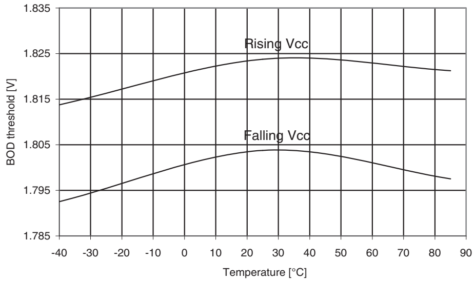
Figure 31-286. ATmega3290A: BOD Thresholds vs. temperature (BOD level is 1.8V).
