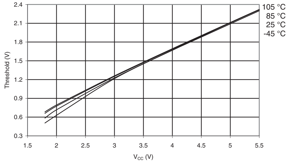
Figure 32-34. ATmega169PA-105°C: I/O Pin Input Threshold Voltage vs. V_{CC} ( V_{IL} , I/O Pin Read as "0")
