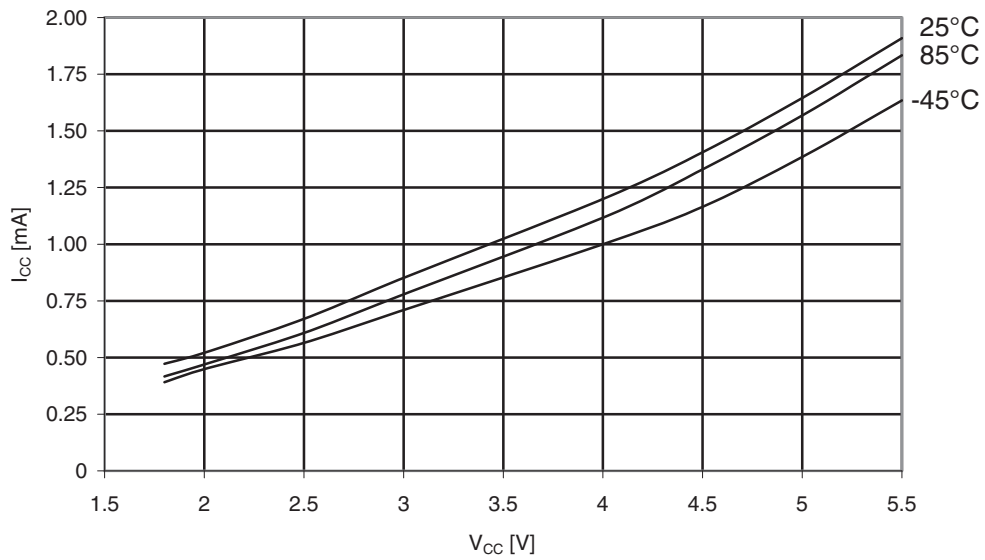
Figure 31-8. Atmega169A: Idle supply current vs. V_{CC} (Internal RC oscillator, 8MHz).
