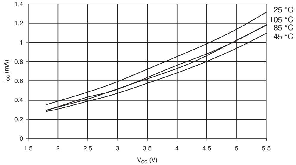
Figure 32-4. ATmega169PA-105°C: Active Supply Current vs. V_{CC} (Internal RC Oscillator, 1MHz)
