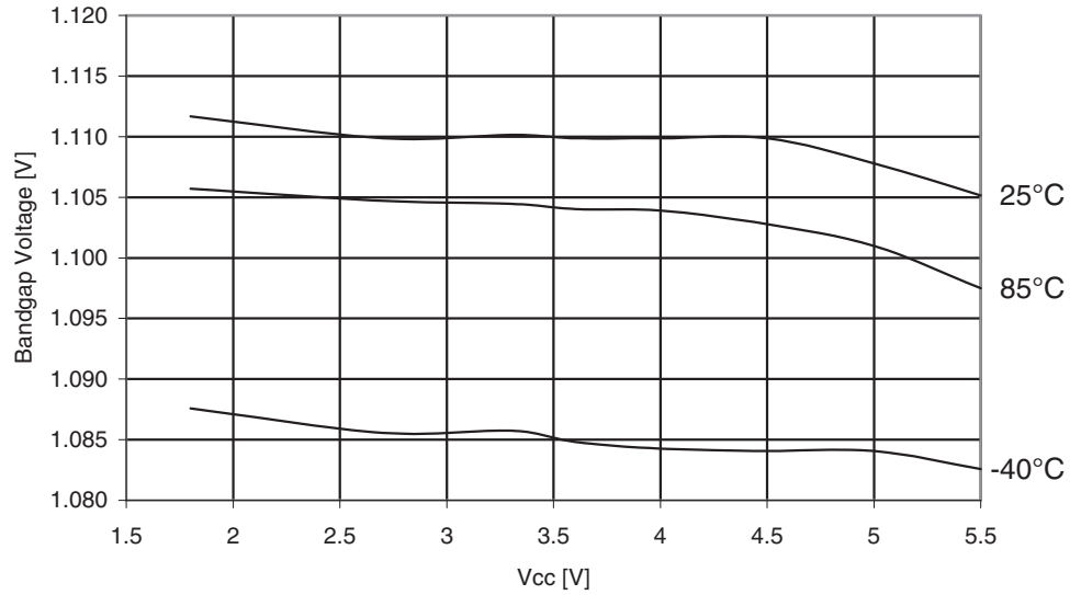
Figure 31-167. Atmel ATmega329A: Bandgap voltage vs. V_{CC} .
