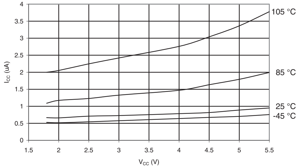
Figure 32-14. ATmega169PA-105°C: Standby Supply Current vs. V_{CC} (32 kHz Watch Crystal, Watchdog Timer Disabled)
