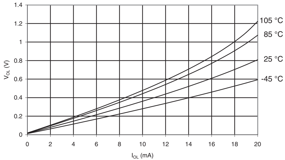
Figure 32-31. ATmega169PA-105°C: I/O Pin Output Voltage vs. Sink Current, Port B ( V_{CC}= 2.7V )
