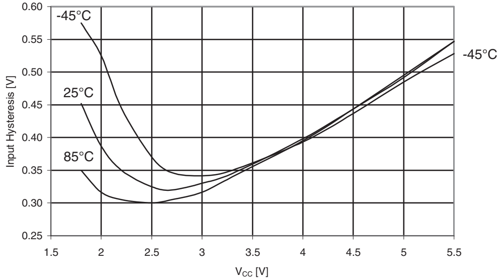
Figure 31-584. Atmel ATmega6490P: I/O pin input Hysteresis vs. V_{CC} .
