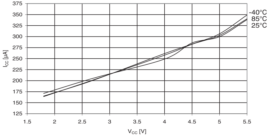
Figure 31-297. Atmel ATmega3290A: Active supply current with ADC at 1MHz vs. V_{CC} .
