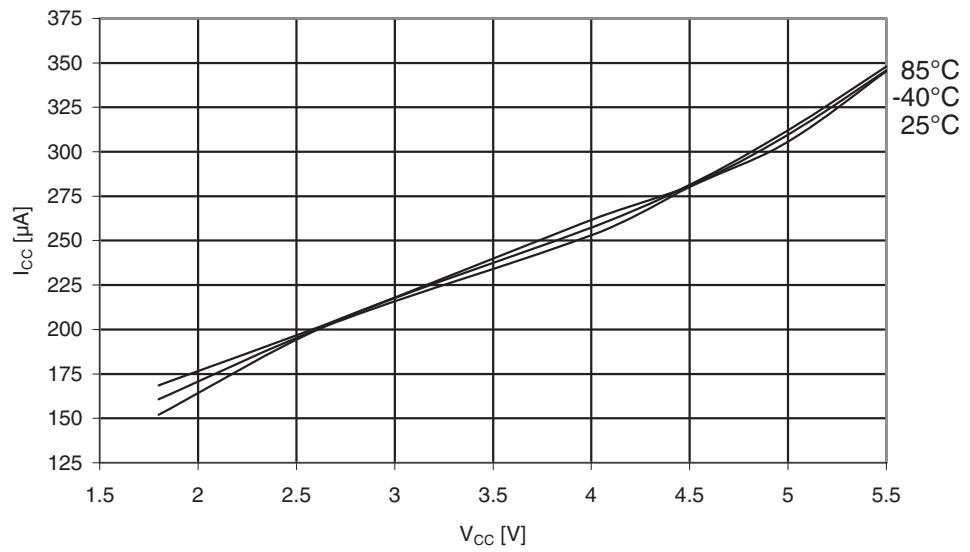
Figure 31-236. ATmega329PA: Active supply current with ADC at 200kHz vs. V_{CC} .
