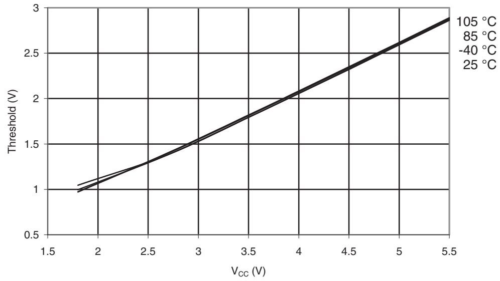
Figure 32-150. ATmega329P-105°C: I/O Pin Input Threshold Voltage vs. V_{CC} ( V_{IH} , I/O Pin Read as “1”)
