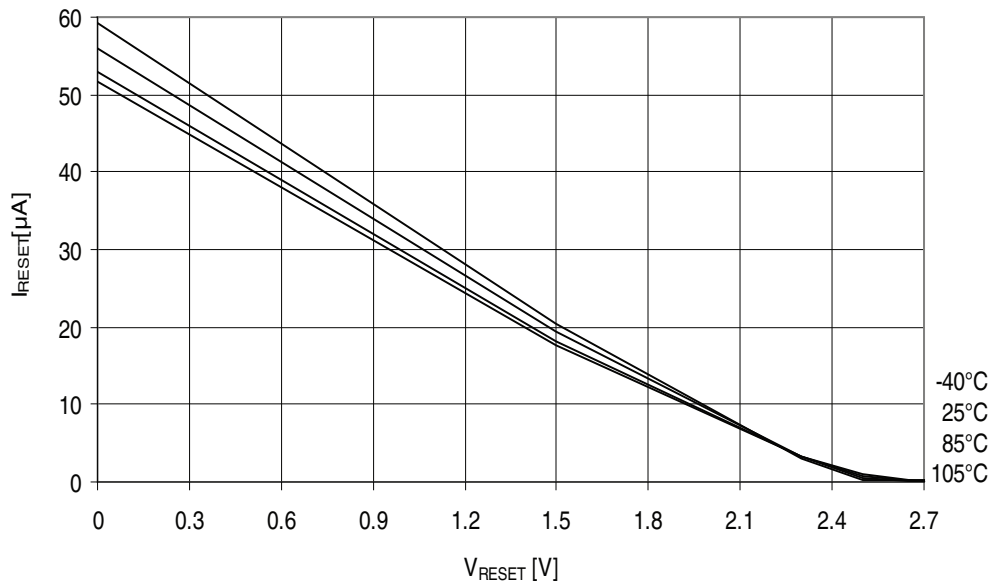
Figure 32-371. ATmega3290PA - 105°C: Reset Pull-up Resistor Current vs. Reset Pin Voltage ( V_{CC} = 2.7V )
