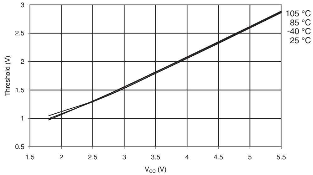
Figure 32-328. ATmega3290PA-105°C: I/O Pin Input Threshold Voltage vs. V_{CC} ( V_{IH} , I/O Pin Read as “1”)
