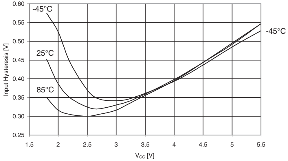
Figure 31-523. Atmel ATmega6490A: I/O pin input Hysteresis vs. V_{CC} .
