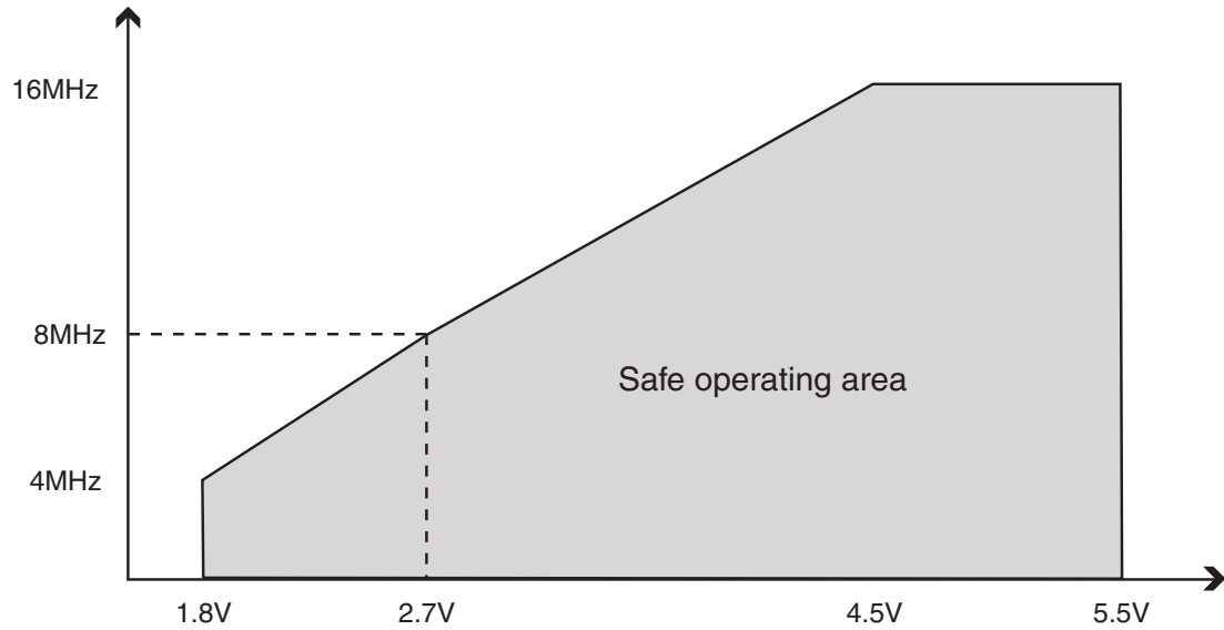
Figure 29-1. Maximum frequency vs. V_{CC} , Atmel ATmega169A/169PA/ATmega649A/ATmega649P.
