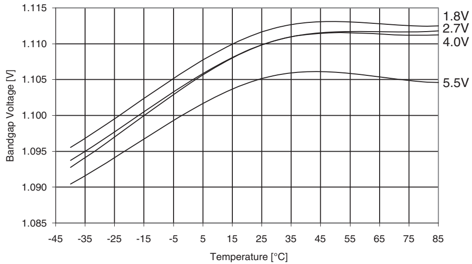
Figure 31-228. ATmega329PA: Bandgap voltage vs. temperature.
