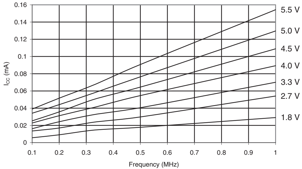
Figure 32-56. ATmega169PA-105°C: Reset Supply Current vs. V_{CC} (0.1 - 1.0 MHz, Excluding Current Through The Reset Pull-up)
