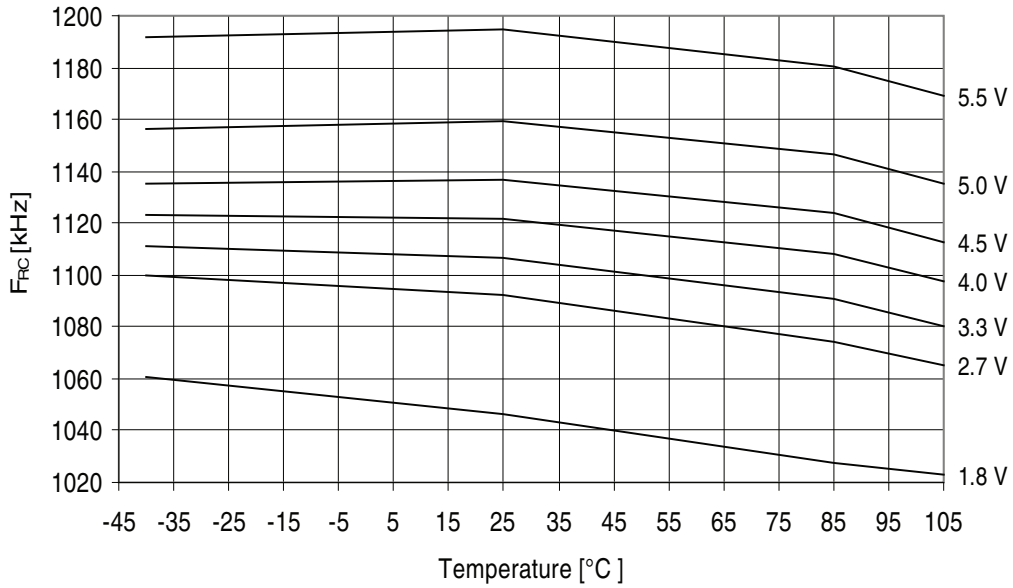
Figure 32-396. ATmega3290PA - 105°C: Watchdog Oscillator Frequency vs. Temperature
