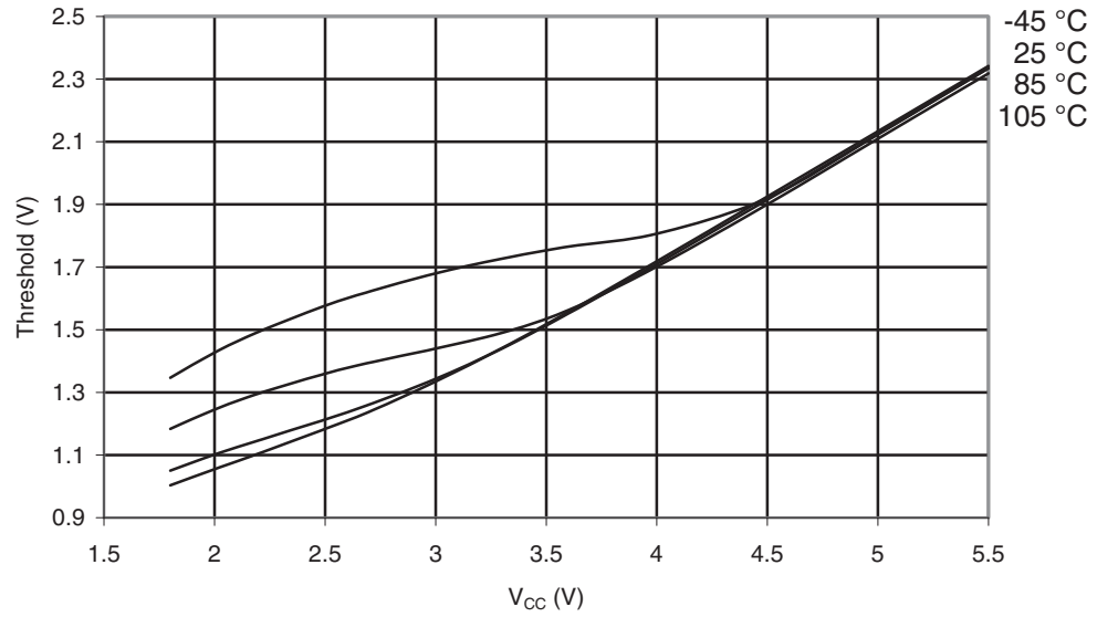
Figure 32-36. ATmega169PA-105°C: Reset Input Threshold Voltage vs. V_{CC} ( V_{IH} , Reset Pin Read as "1")
