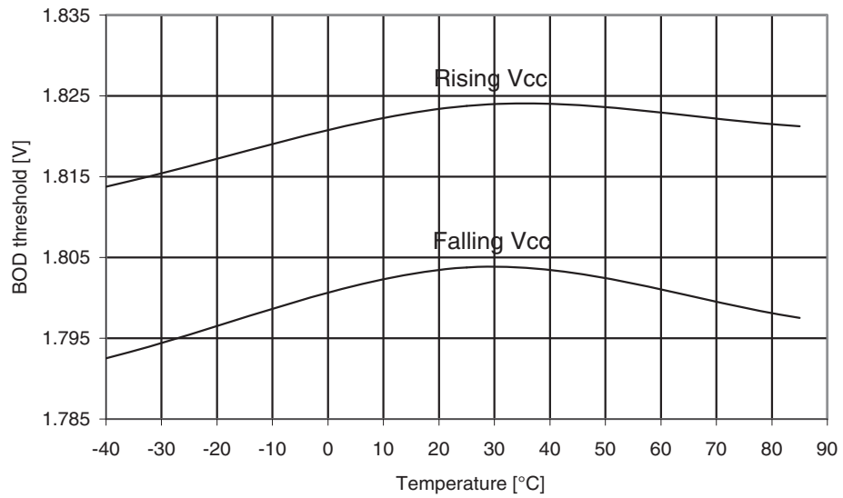
Figure 31-226. ATmega329PA: BOD Thresholds vs. temperature (BOD level is 1.8V).
