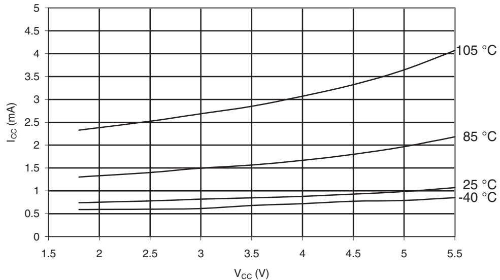
Figure 32-135. ATmega329P-105°C: Standby Supply Current vs. V_{CC} (32kHz Watch Crystal, Watchdog Timer Disabled)
