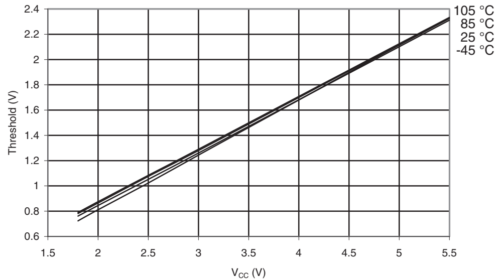
Figure 32-37. ATmega169PA-105°C: Reset Input Threshold Voltage vs. V_{CC} ( V_{IL} , Reset Pin Read as "0")
