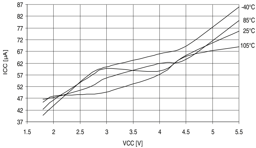
Figure 32-231. ATmega329PA - 105°C: Analog Comparator Current vs. V_{CC}
