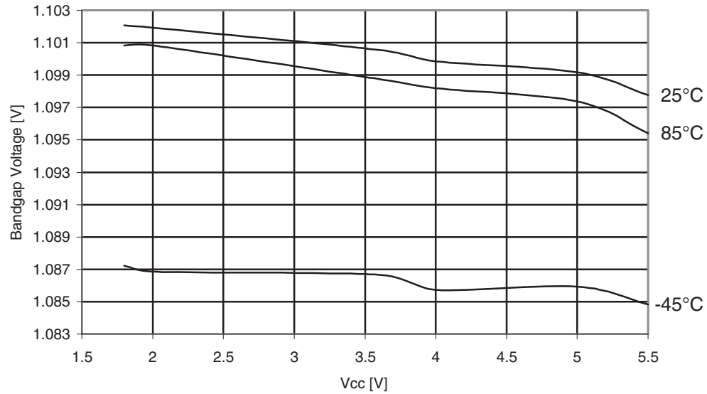
Figure 31-591. ATmega6490P: Bandgap voltage vs. V CC .
