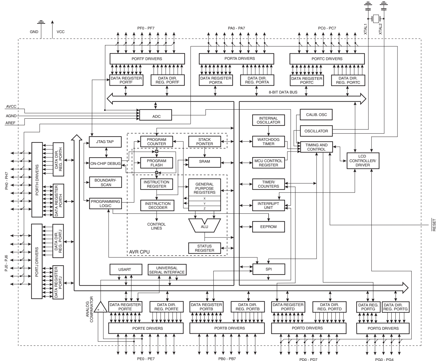
Figure 2-1. Block diagram.
