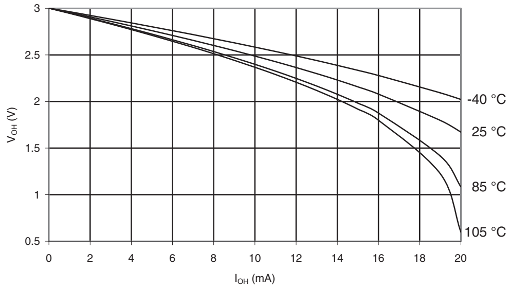
Figure 32-145. ATmega329P-105°C: I/O Pin Output Voltage vs. Source Current, Port B ( V_{CC} = 3V )
