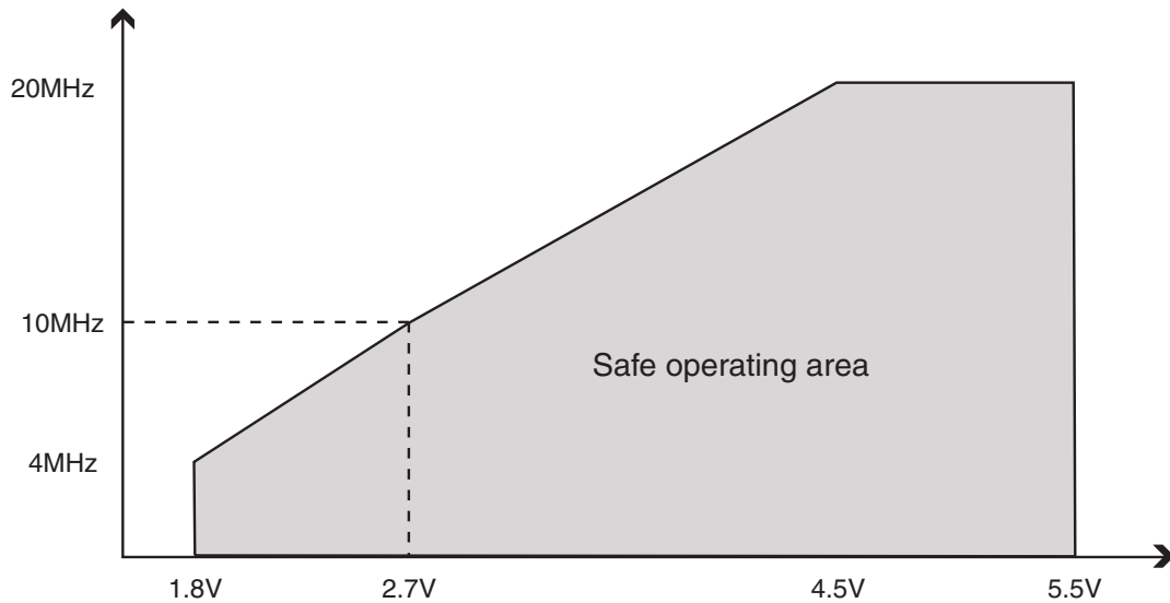
Figure 29-2. Maximum frequency vs. V_{CC} (0 - 20MHz) Atmel ATmega329A/ATmega329PA/ATmega3290A/ATmega3290PA/ATmega6490A/ATmega6490P.
