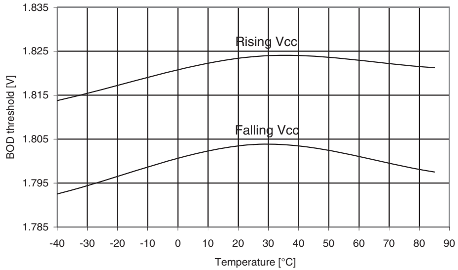
Figure 31-166. ATmega329A: BOD Thresholds vs. temperature (BOD level is 1.8V).
