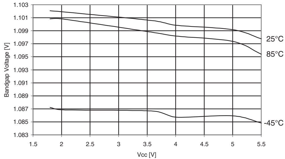
Figure 31-408. ATmega649A: Bandgap voltage vs. V CC .
