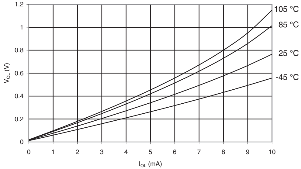
Figure 32-28. ATmega169PA-105°C: I/O Pin Output Voltage vs. Sink Current, Ports A, C, D, E, F, G ( V_{CC} = 2.7V )
