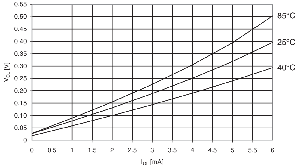
Figure 31-337. ATmega3290PA: I/O pin output voltage vs. sink current, port B ( V_{CC} = 1.8V ).
