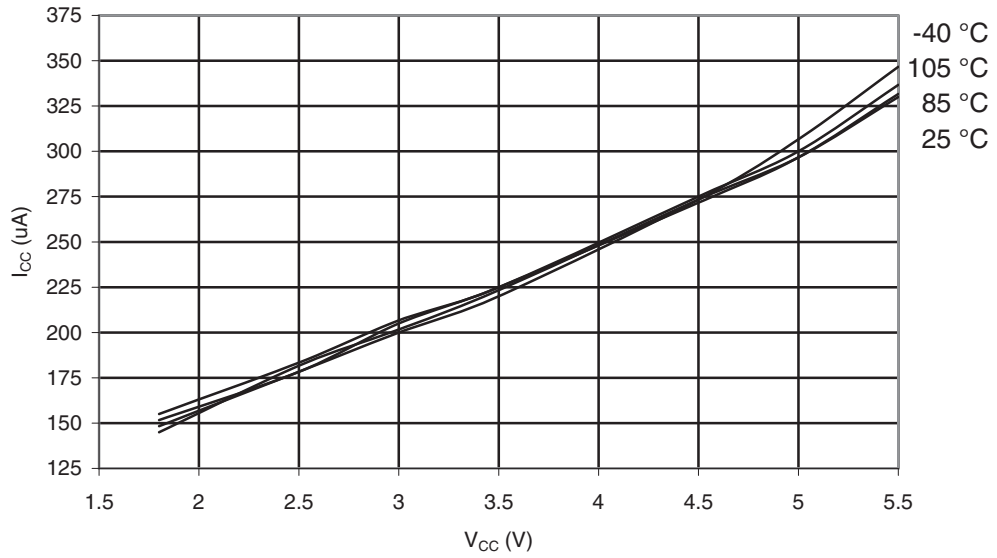
Figure 32-166. ATmega329P-105°C: Active supply current with ADC vs. V_{CC}
