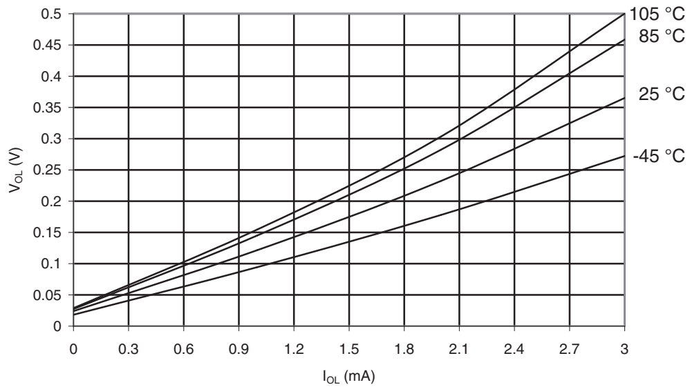
Figure 32-29. ATmega169PA-105°C: I/O Pin Output Voltage vs. Sink Current, Ports A, C, D, E, F, G ( V_{CC} = 1.8V )
