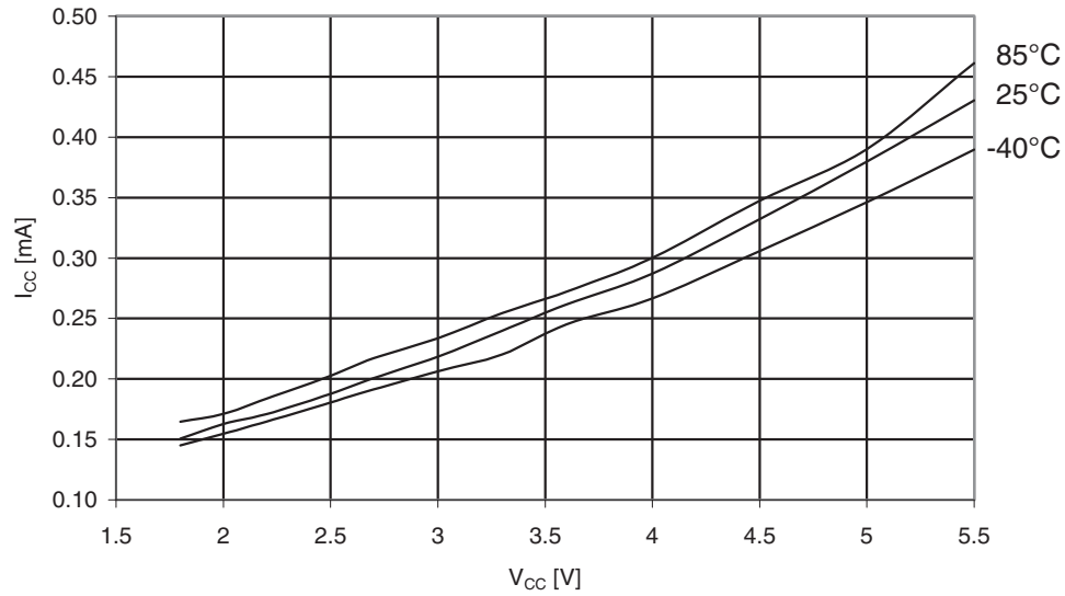
Figure 31-133. Atmel ATmega329A: Idle supply current vs. V_{CC} (Internal RC oscillator, 1MHz).
