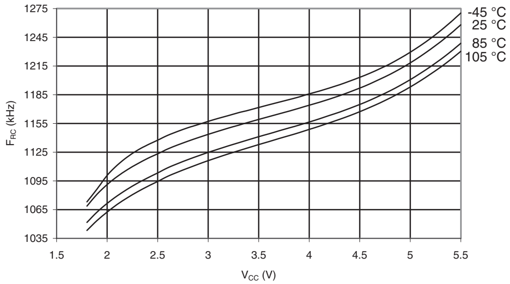
Figure 32-44. ATmega169PA-105°C: Watchdog Oscillator Frequency vs. V_{CC}
