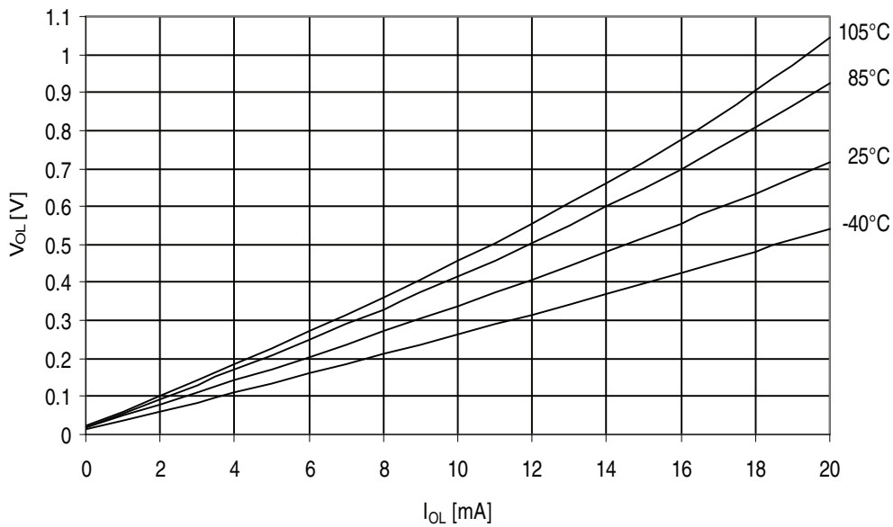
Figure 32-383. ATmega3290PA - 105°C: I/O Pin Output Voltage vs. Sink Current, Port B ( V_{CC} = 3V )
