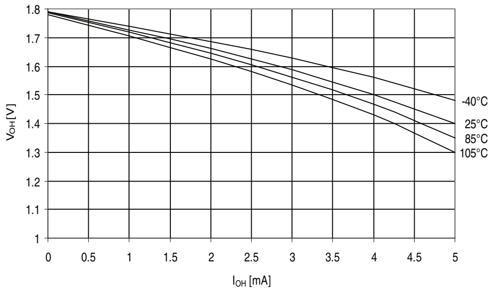
Figure 32-199. ATmega329PA - 105°C: I/O Pin Output Voltage vs. Source Current, Port B ( V_{CC} = 1.8V )
