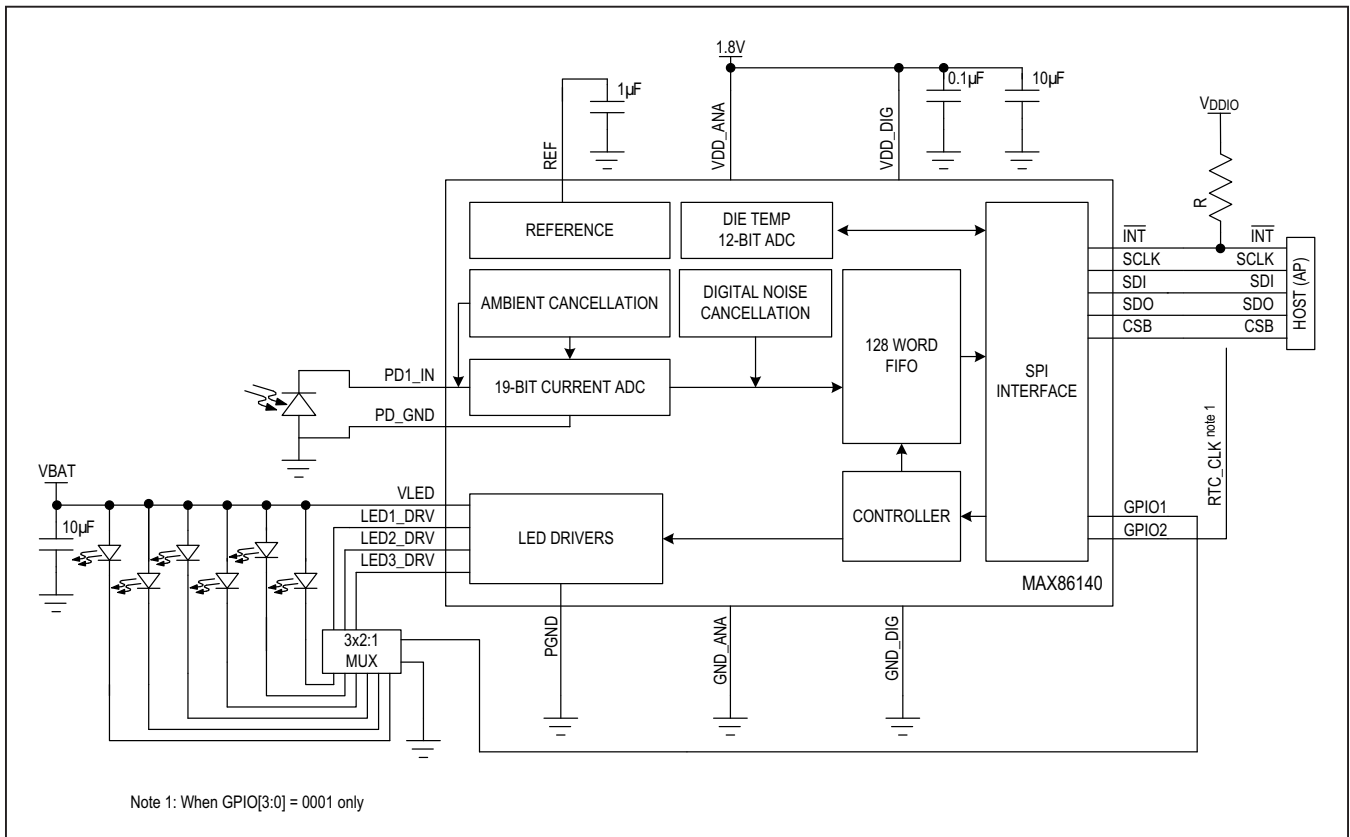
Figure 9. Block Diagram for GPIO CTRL[3:0] 0000 and 0001 With External Mux
