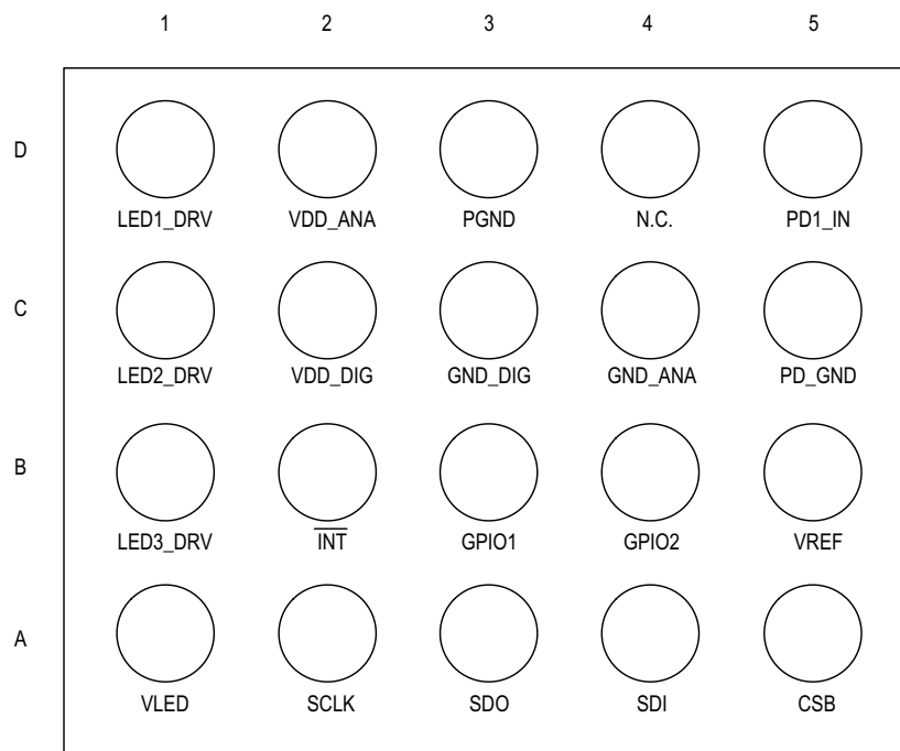
BUMPS FACING UP, 0.4MM PITCH
