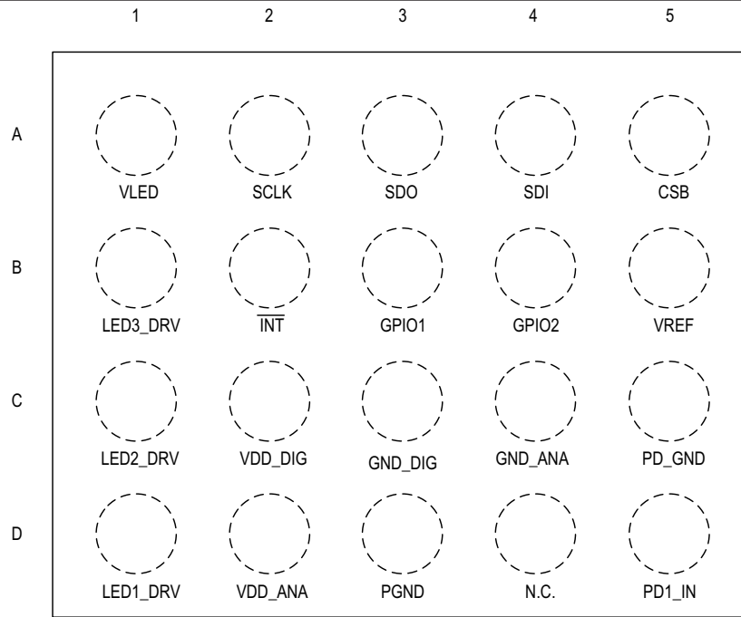
BUMPS FACING DOWN, 0.4MM PITCH
