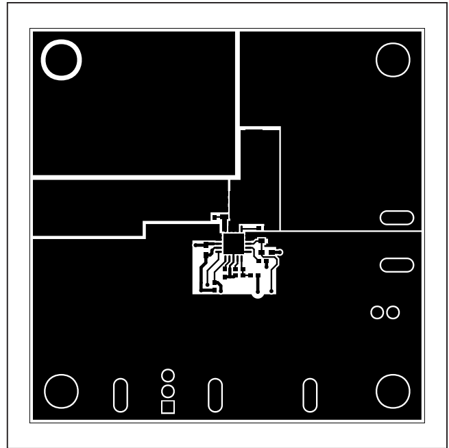
MAX17506 3.3V Output EV Kit PCB Layout—Component Side
