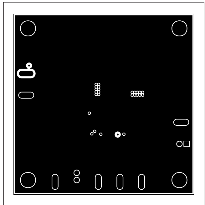
MAX17506 3.3V Output EV Kit PCB Layout—Inner-Layer 2
