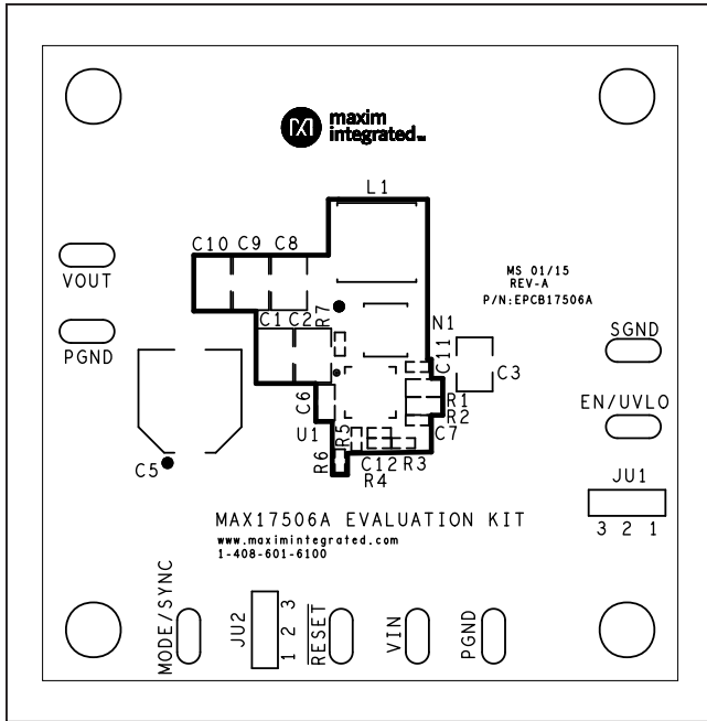
MAX17506 3.3V Output EV Kit Component Placement Guide—Component Side
