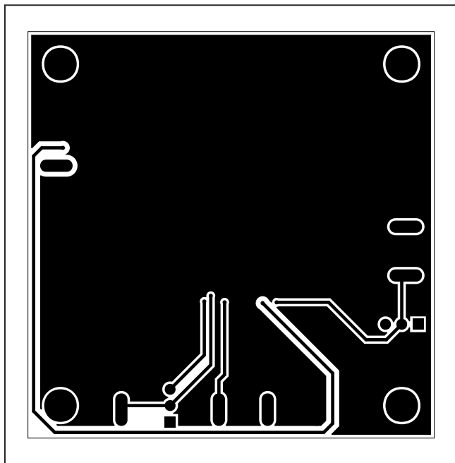
MAX17506 3.3V Output EV Kit PCB Layout—Solder Side
