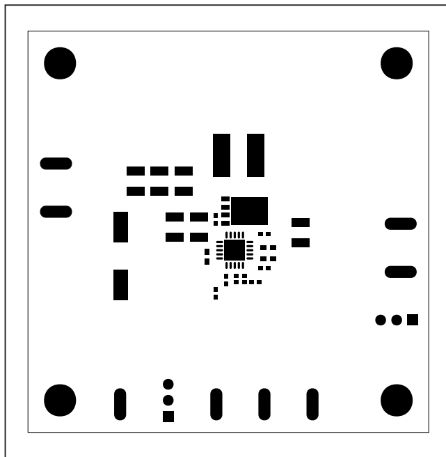
MAX17506 3.3V Output EV Kit Component Placement Guide—Solder Mask
