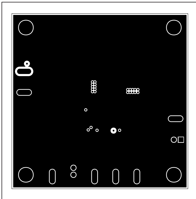
MAX17506 3.3V Output EV Kit PCB Layout—Inner-Layer 1
