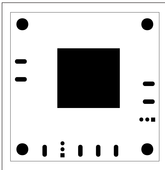
MAX17506 3.3V Output EV Kit Component Placement Guide—Bottom Solder Mask
