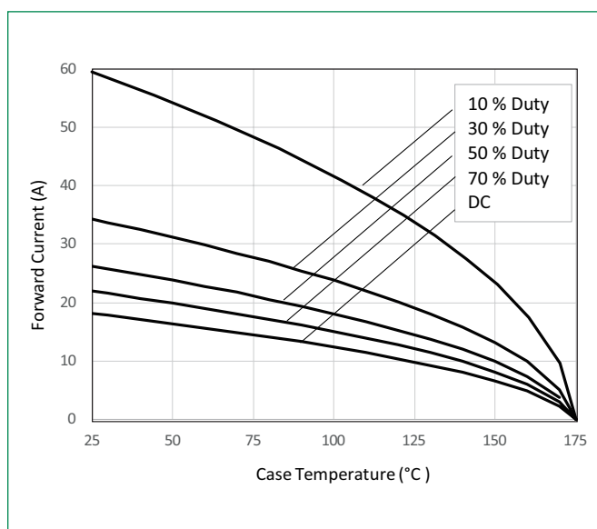
Figure 4: Current Derating
