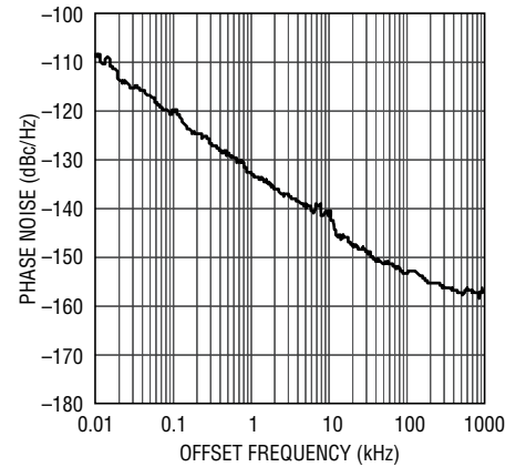
Additive Phase Noise, f_{OUT} = 65MHz , f_{DAC} = 2.7Gsp
