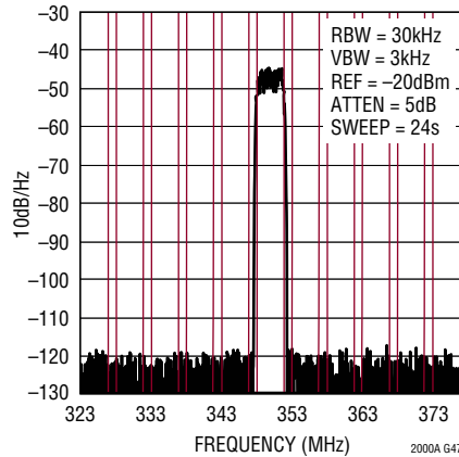
LTC2000A-16 Single Carrier WCDMA ACLR at 350MHz, f_{DAC} = 2.7Gsp
