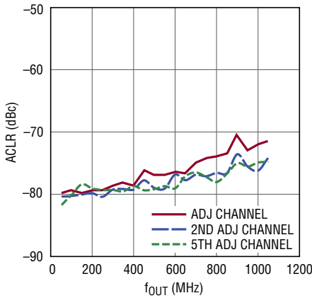
LTC2000A-16 Single Carrier WCDMA ACLR vs f_{OUT} , f_{DAC} = 2.7Gsp
