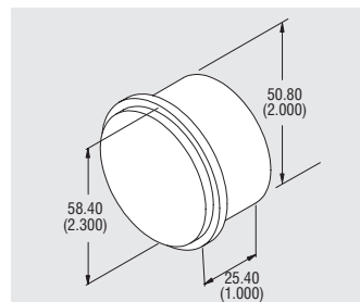
Panel Cutout: 52.3 (2.060) Approximate in mm (inches).
