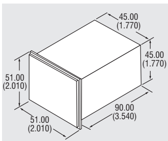
Panel Cutout: 45 x 45 (1.770 x 1.770) Approximate in mm (inches).
