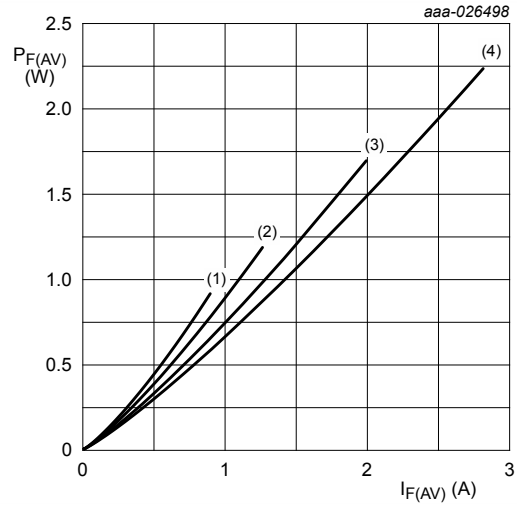
Fig. 6. Average forward power dissipation as a function of average forward current; typical values T_j = 150\text{ °C} (1) \delta = 0.1 (2) \delta = 0.2 (3) \delta = 0.5 (4) \delta = 1 (DC)
