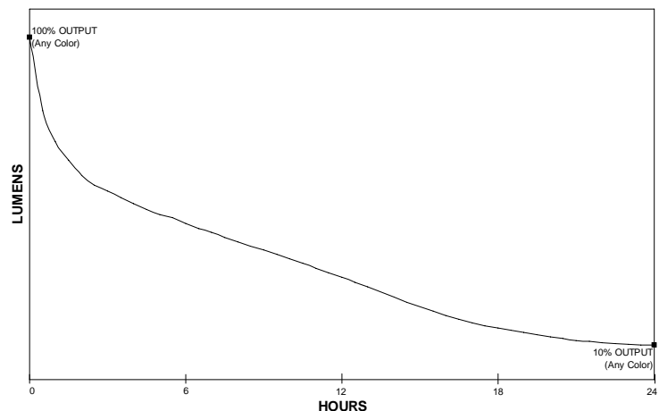
PERFORMANCE CURVE
