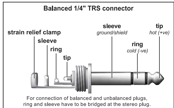
Fig. 4.3: 1/4" stereo plug
