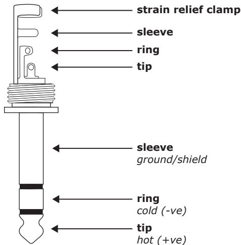
Fig. 2.1: XLR Balanced
