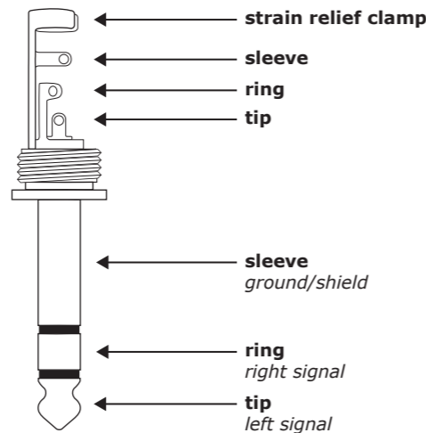
Fig. 3.3: 1/4" TRS connector
