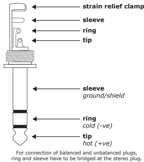
Fig. 3.3: 1/4" TRS connector
