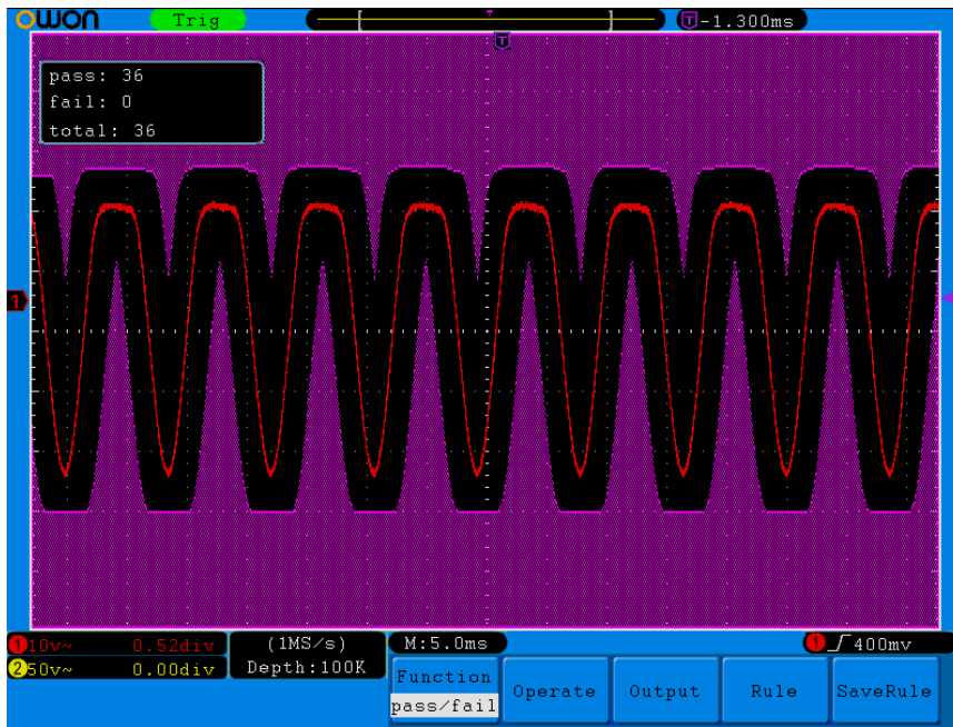
Figure 5-55 Pass/Fail test
