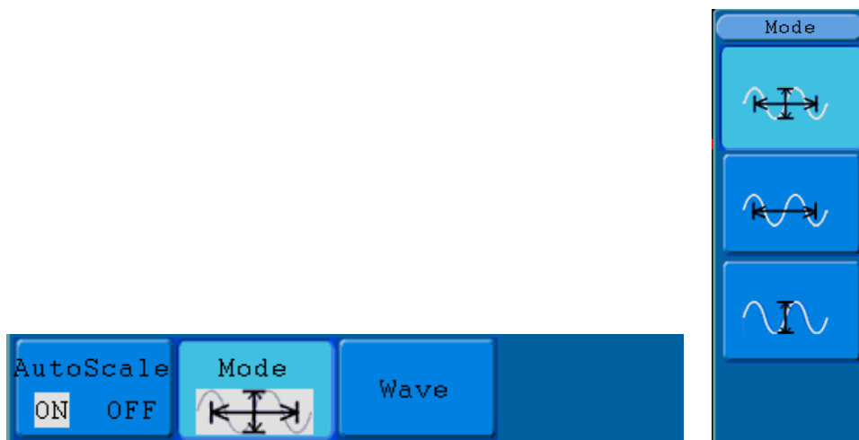
Figure 5-68 Autoscale menu
