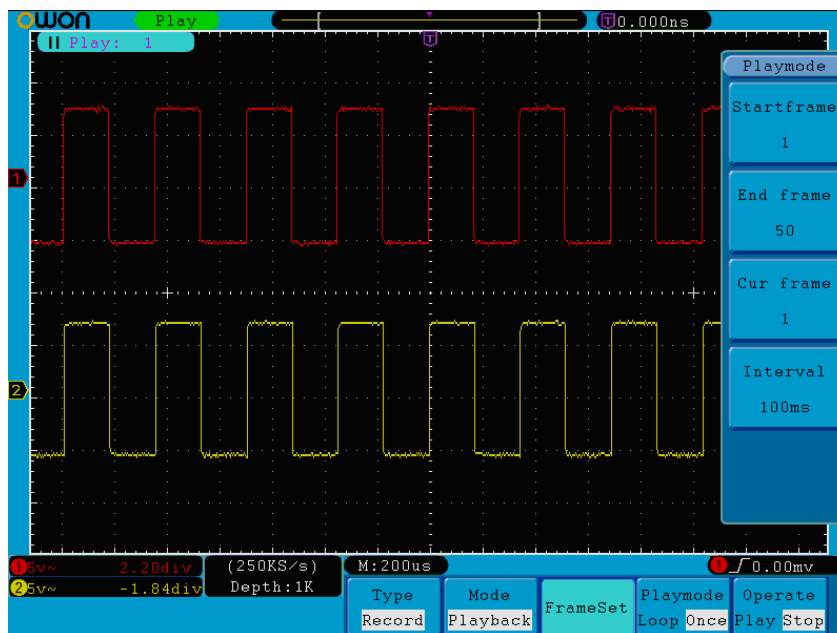
Figure 5-48 Wave Playback
