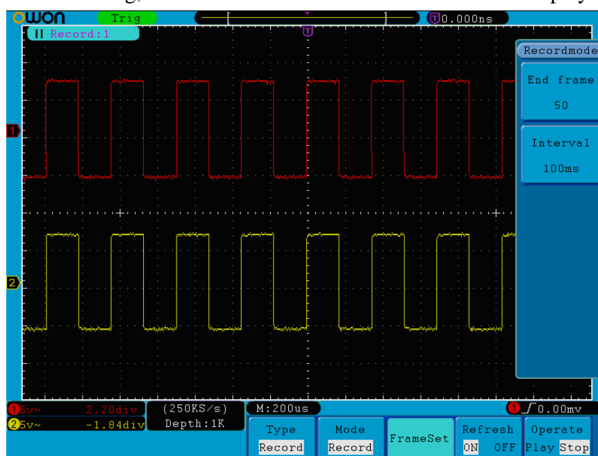
Figure 5-47 Wave Record
