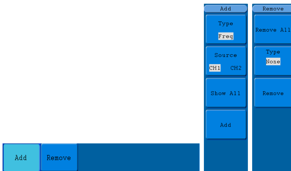
Figure 5-58 Measure Menu
