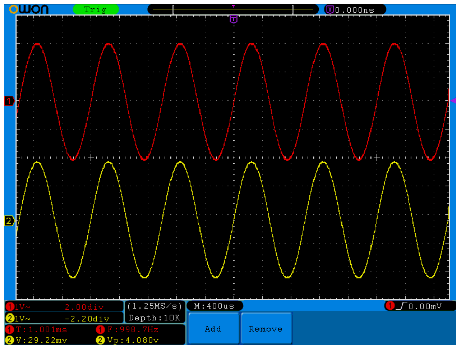
Figure 5-59 automatic measurement
