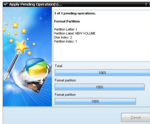
Figure 5-45: Format process
