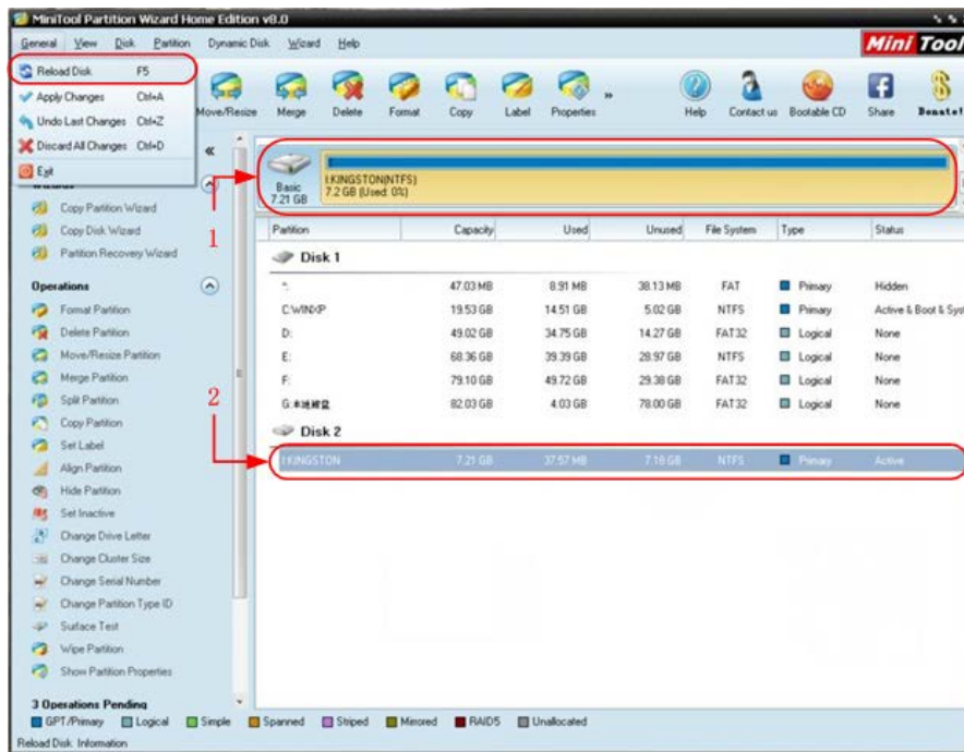
Figure 5-41: Reload Disk
