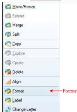
Figure 5-42: Choose format
