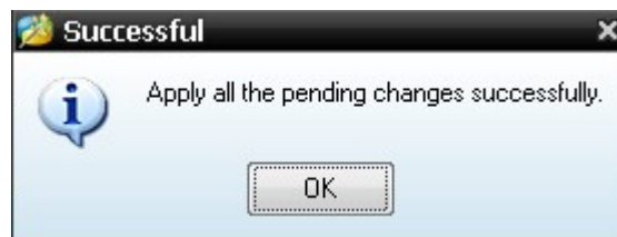
Figure 5-46: Format successfully
