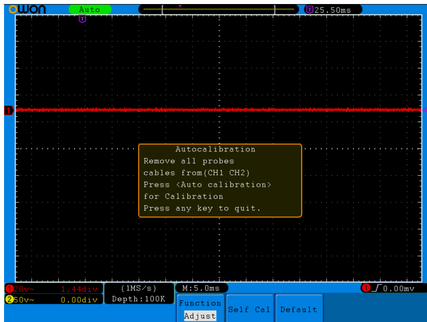
Figure 5-53 Self-Calibration
