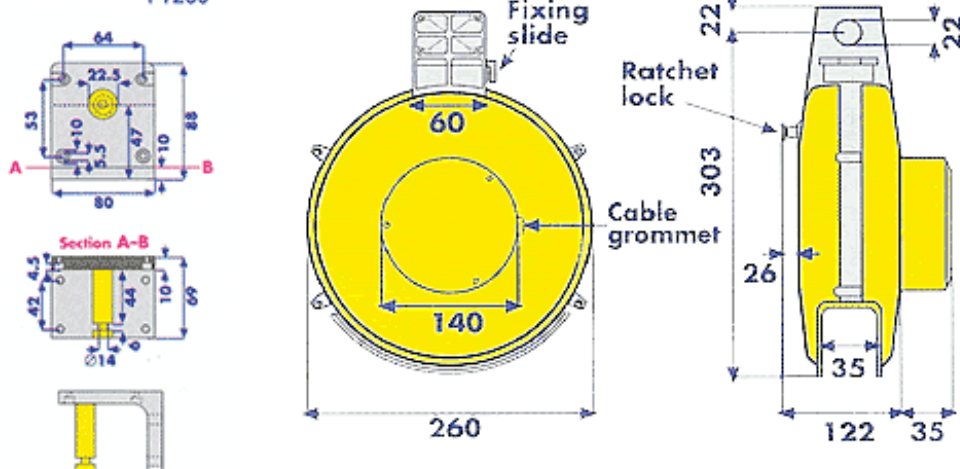
Universal bracket for FT260
