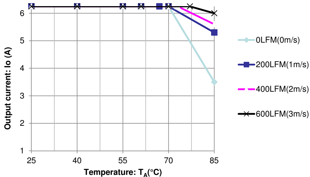
Figure 16 AVD75B-48S12-6L and AVD75B-48S12TL
