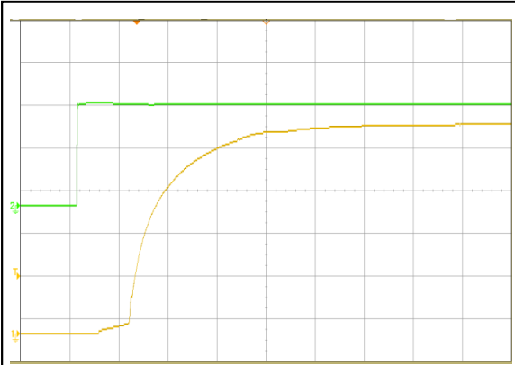
Figure 1: AVD75B-48S05 Output Voltage Startup Characteristic (10ms/div) Ch 1: Vo (1V/div) Ch 2: Vin (20V/div)
