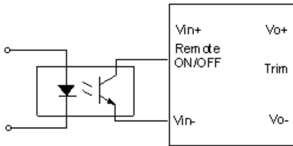
Isolated remote ON/OFF circuit
