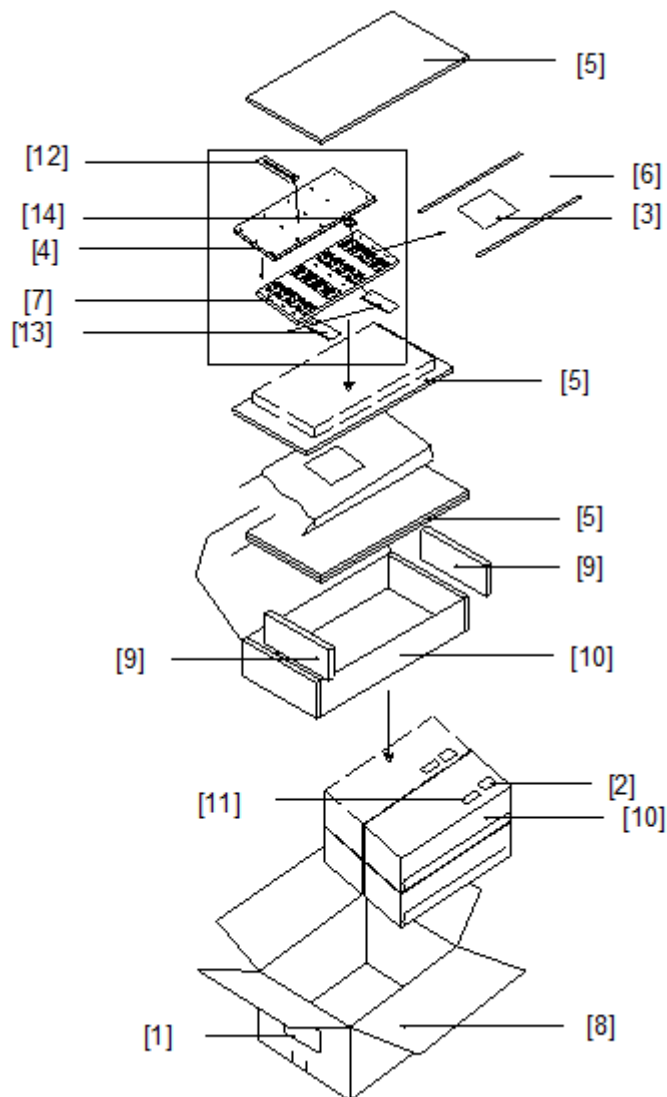
Figure 23 Package disassembly
