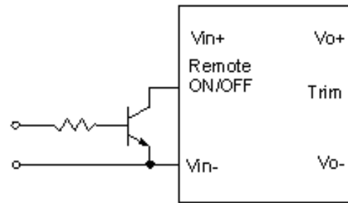
Non-isolated remote ON/OFF circuit
