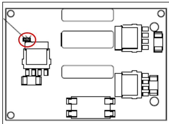
Figure 10: AVD75B-48S3V3 OTP test point (Open-frame module)
