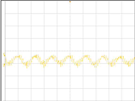
Figure 1: AVD75B-48S3V3 Input Reflected Ripple Current Waveform Ch 1: Iin (2uS/div, 10mA/div)
