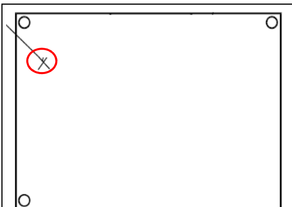
Figure 11: AVD75B-48S3V3 OTP test point (Module with baseplate)
