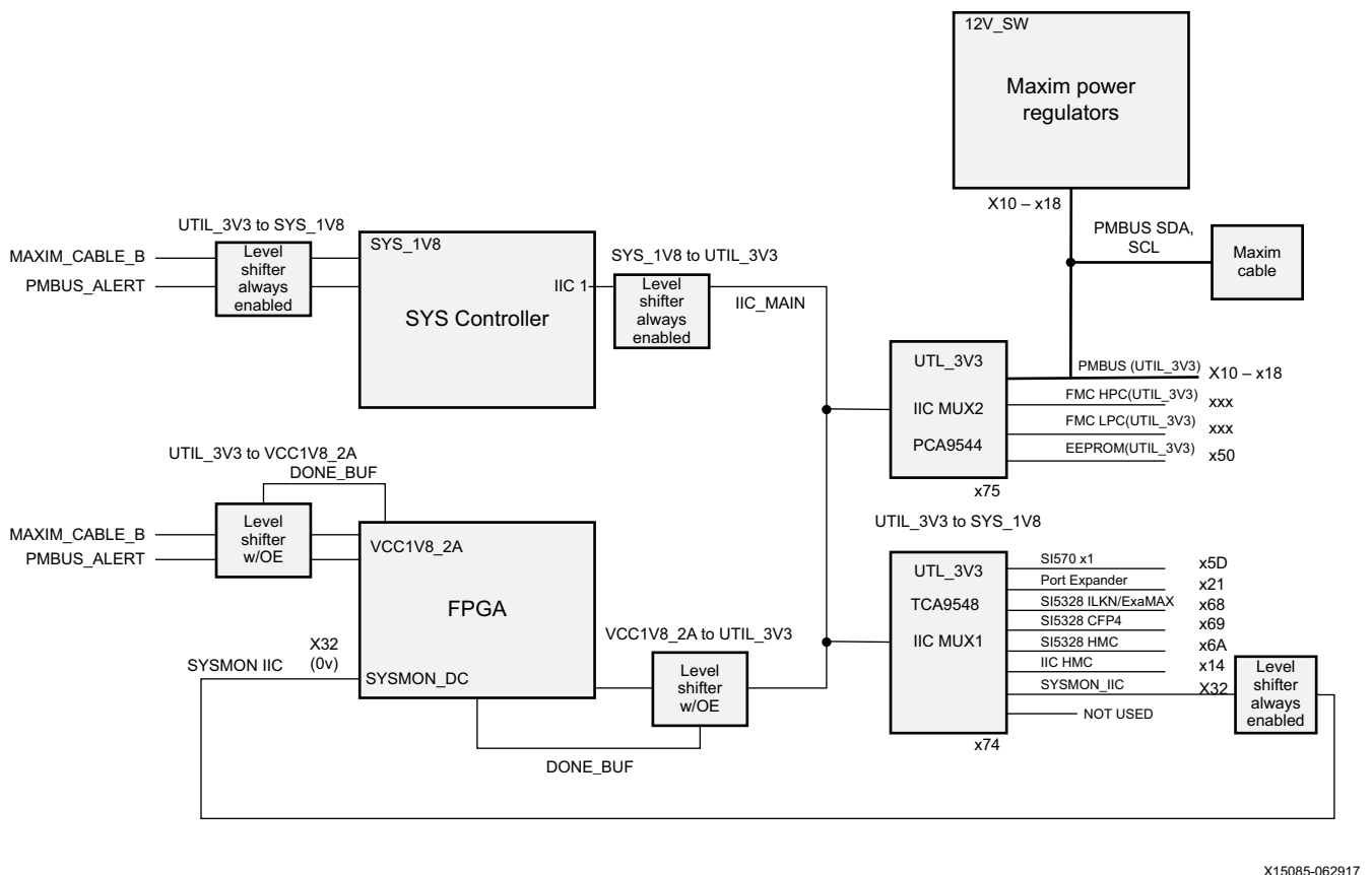
Figure 1-16: I2C Bus Topology Overview
