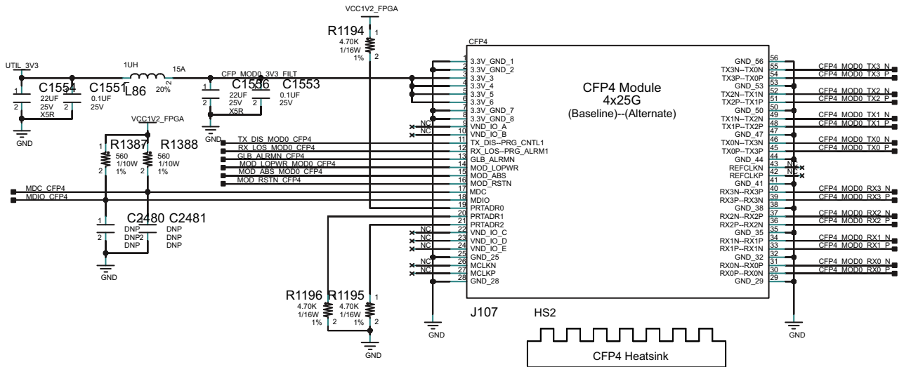
Figure 1-14: CFP Module Connector Circuit
