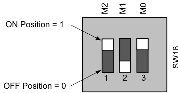
Figure 1-3: SW16 Default Settings
